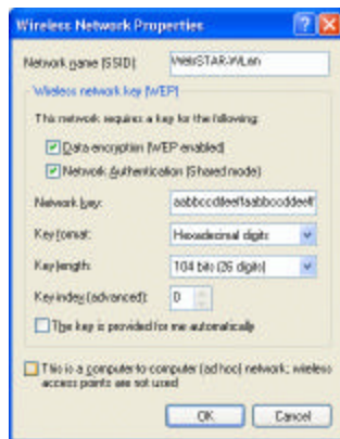
Figure 3-15 Windows XP-Add Preferred Networks
