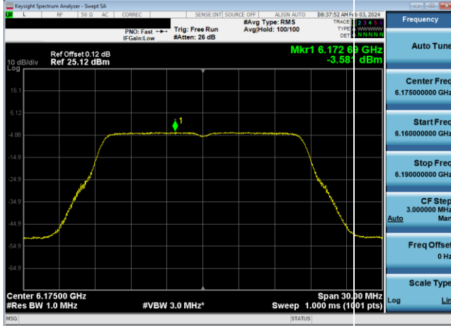
Plot 7-181. Power Spectral Density Plot Antenna WF5B LPI (20MHz 802.11a (UNII Band 5) – Ch. 45, 12Mbps)
