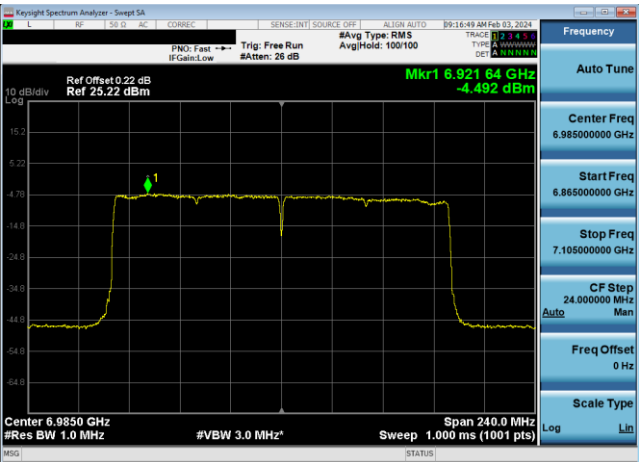
Plot 7-200. Power Spectral Density Plot Antenna WF5B LPI (160MHz 802.11ax (UNII Band 8) – Ch. 207, MCS2)
