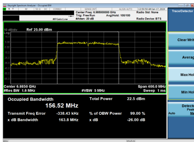
Plot 7-180. 26dB & 99% Bandwidth Plot Antenna WF7 (160MHz 802.11ax (UNII Band 8) – Ch. 207, MCS11)
