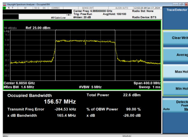
Plot 7-160. 26dB & 99% Bandwidth Plot Antenna WF7 (160MHz 802.11ax (UNII Band 8) – Ch. 207, MCS4)
