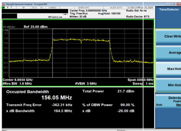
Plot 7-155. 26dB & 99% Bandwidth Plot Antenna WF7 (160MHz 802.11ax (UNII Band 7) – Ch. 143, MCS4)
