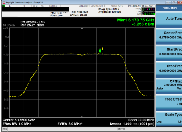
Plot 7-201. Power Spectral Density Plot Antenna WF5B LPI (20MHz 802.11a (UNII Band 5) – Ch. 45, 24Mbps)
