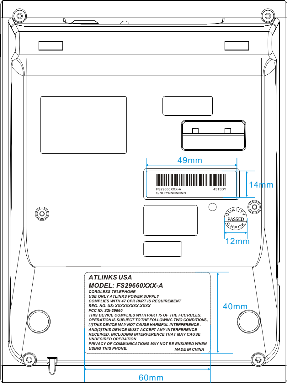
Base unit
