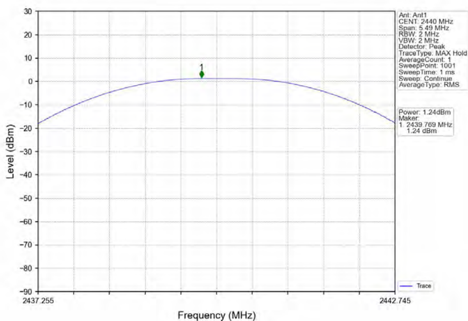
8-DPSK_MCH_2440MHz_Ant1_NTNV
