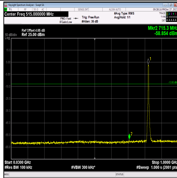
Band5-4132-2-30~1000MHz-PASS
