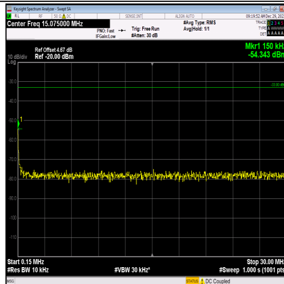
Band4-1413-3-0.15~30MHz-PASS
