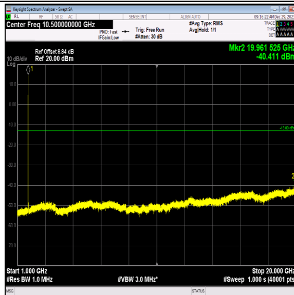
Band4-1413-2-1000~20000MHz-PASS
