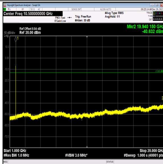
Band4-1513-4-1000~20000MHz-PASS
