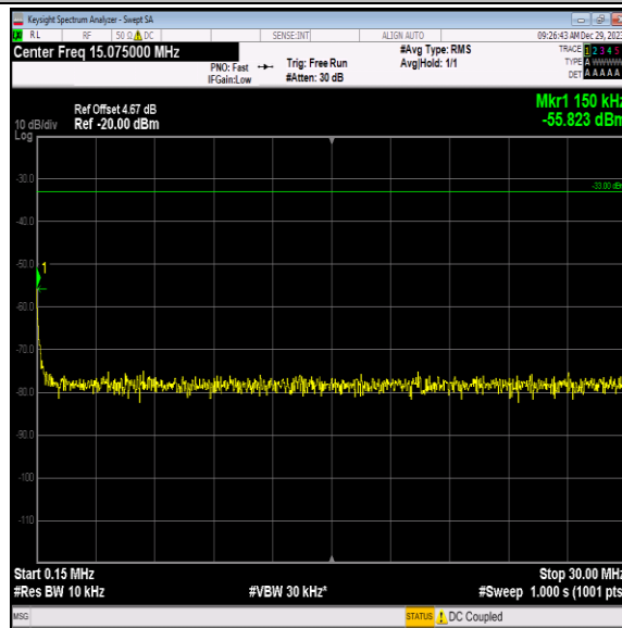
Band4-1413-5-0.15~30MHz-PASS
