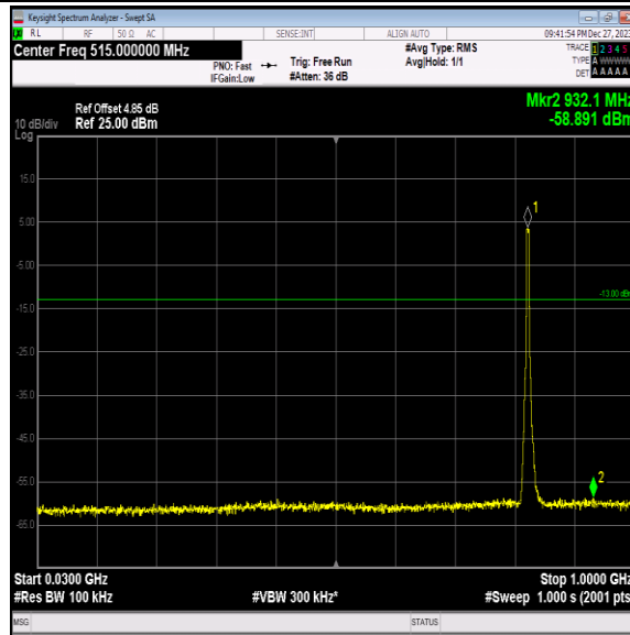
Band5-4132-3-30~1000MHz-PASS
