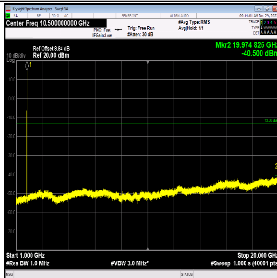
Band4-1513-1-1000~20000MHz-PASS
