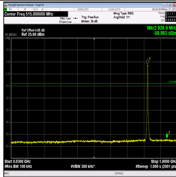
Band5-4132-1-30~1000MHz-PASS
