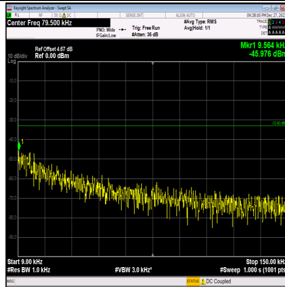
Band5-4132-2-0.009~0.15MHz-PASS
