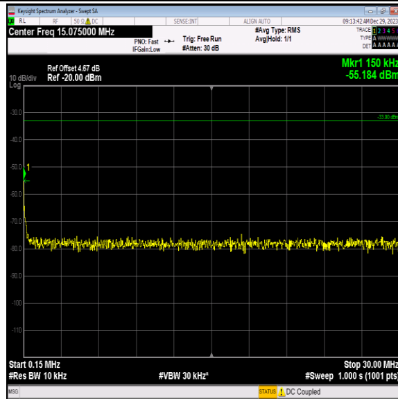
Band4-1513-1-0.15~30MHz-PASS
