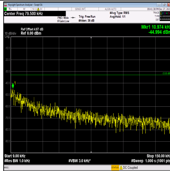
Band5-4132-3-0.009~0.15MHz-PASS
