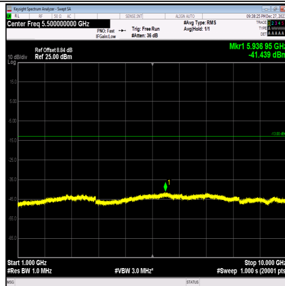
Band5-4132-2-1000~10000MHz-PASS
