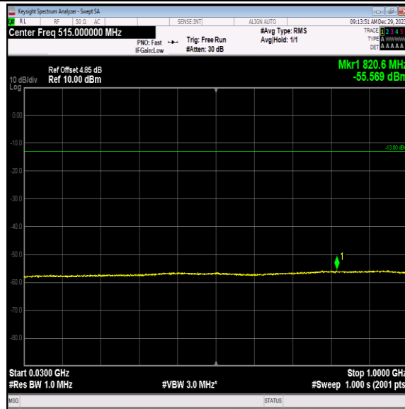
Band4-1513-1-30~1000MHz-PASS
