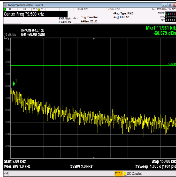
Band4-1413-2-0.009~0.15MHz-PASS
