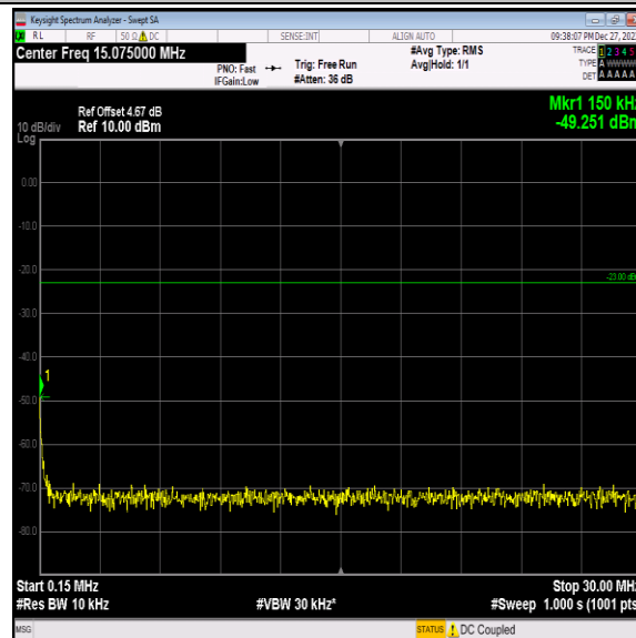
Band5-4132-2-0.15~30MHz-PASS
