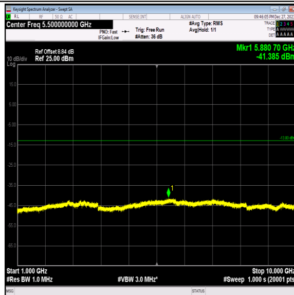
Band5-4132-4-1000~10000MHz-PASS
