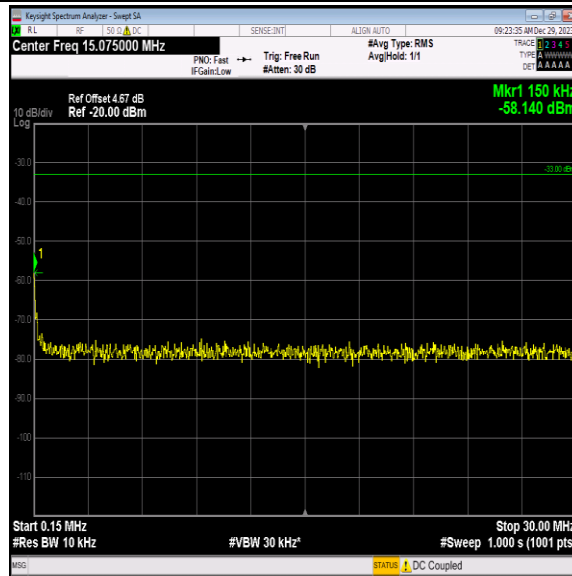
Band4-1413-4-0.15~30MHz-PASS
