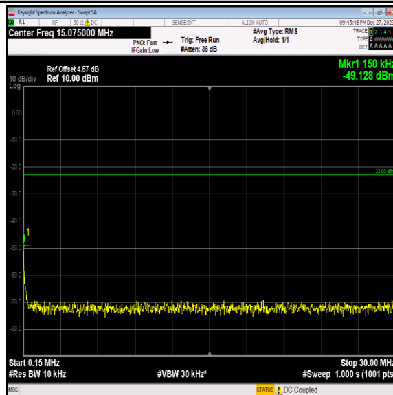
Band5-4132-4-0.15~30MHz-PASS
