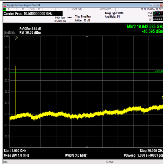
Band4-1513-3-1000~20000MHz-PASS
