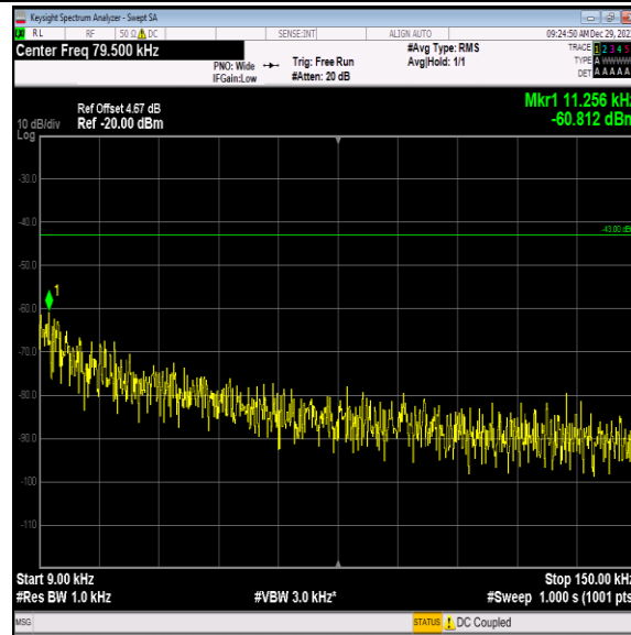
Band4-1513-4-0.009~0.15MHz-PASS
