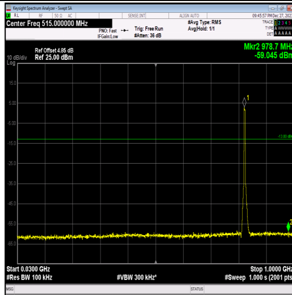
Band5-4132-4-30~1000MHz-PASS
