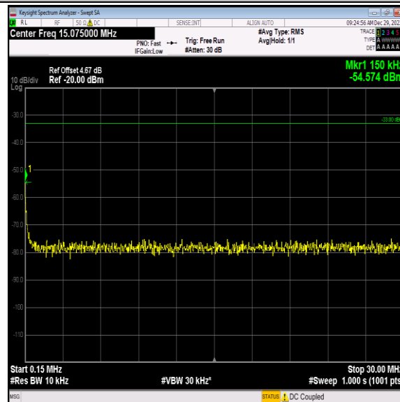
Band4-1513-4-0.15~30MHz-PASS
