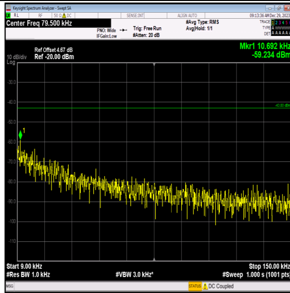
Band4-1513-1-0.009~0.15MHz-PASS
