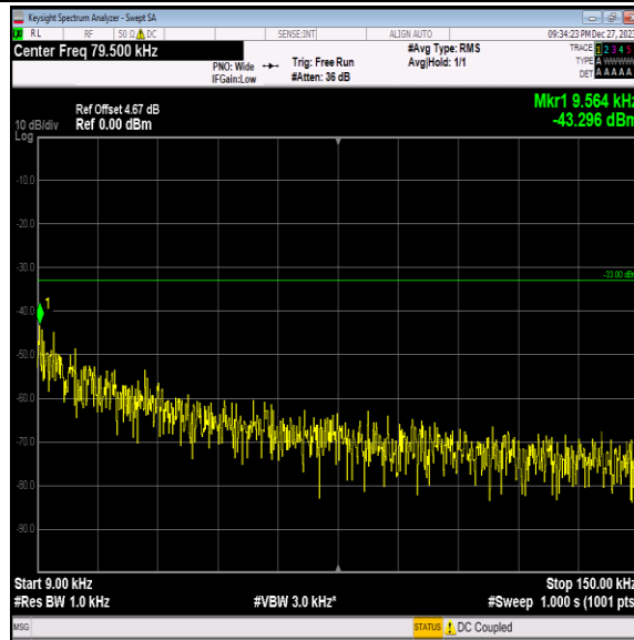
Band5-4132-1-0.009~0.15MHz-PASS
