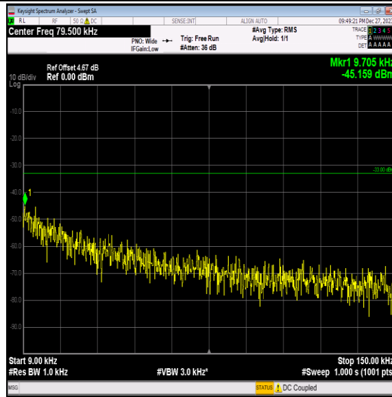
Band5-4132-5-0.009~0.15MHz-PASS
