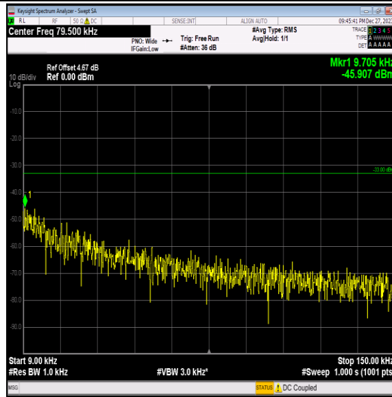
Band5-4132-4-0.009~0.15MHz-PASS
