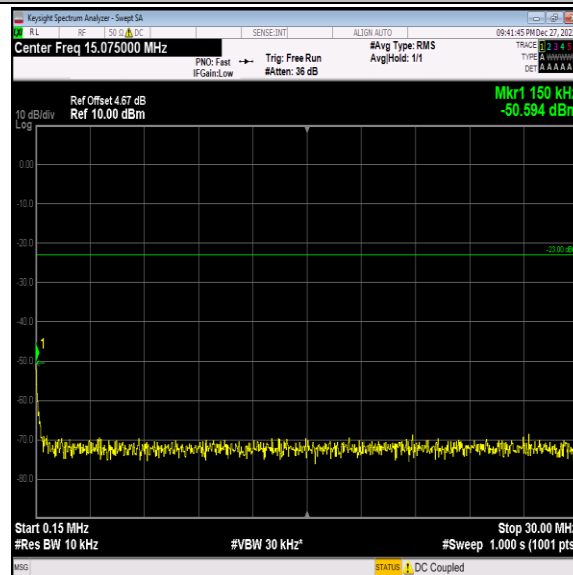
Band5-4132-3-0.15~30MHz-PASS
