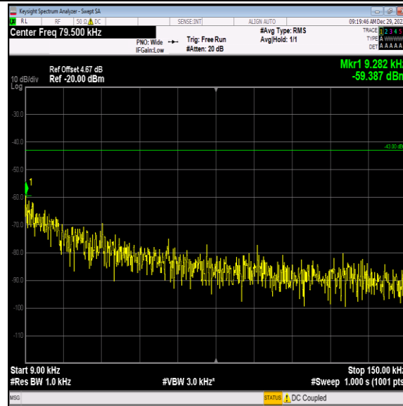
Band4-1413-3-0.009~0.15MHz-PASS
