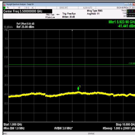
Band5-4132-1-1000~10000MHz-PASS
