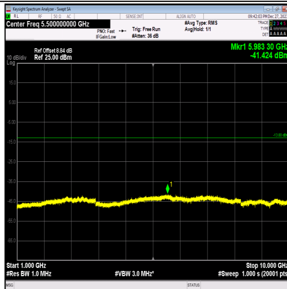
Band5-4132-3-1000~10000MHz-PASS
