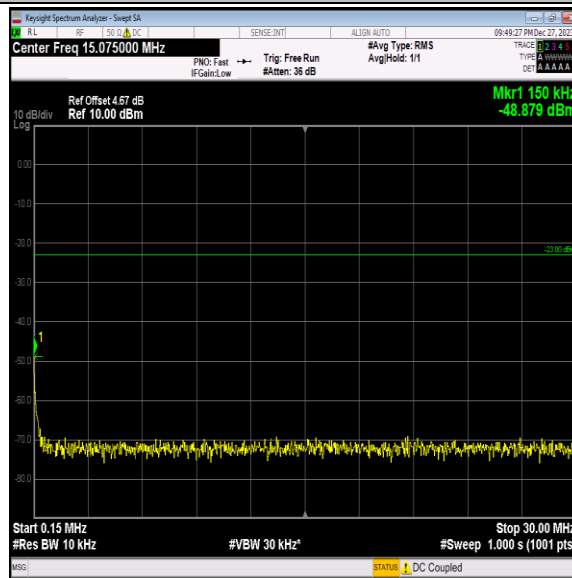
Band5-4132-5-0.15~30MHz-PASS
