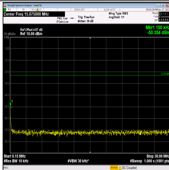
Band5-4132-1-0.15~30MHz-PASS
