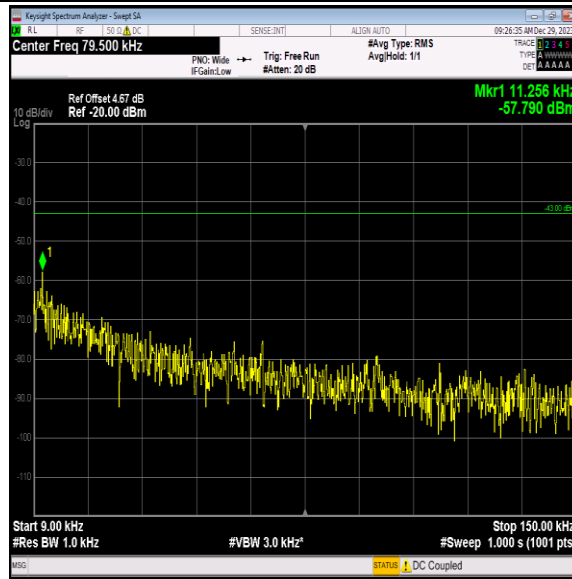
Band4-1413-5-0.009~0.15MHz-PASS
