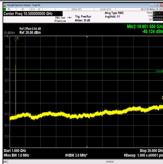
Band4-1513-2-1000~20000MHz-PASS
