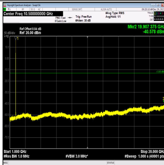
Band4-1413-3-1000~20000MHz-PASS
