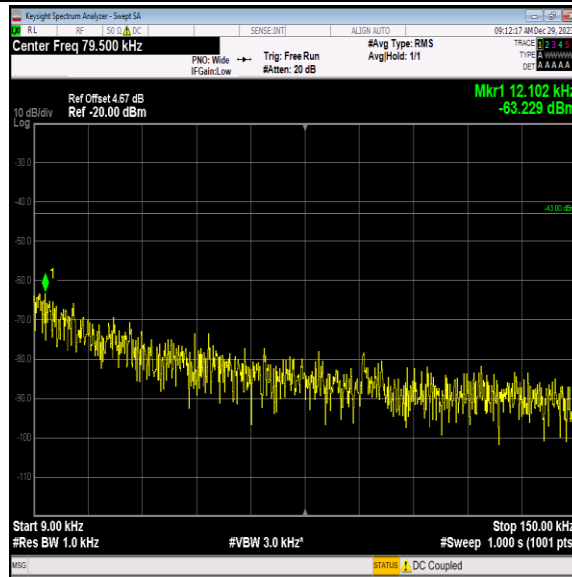
Band4-1413-1-0.009~0.15MHz-PASS
