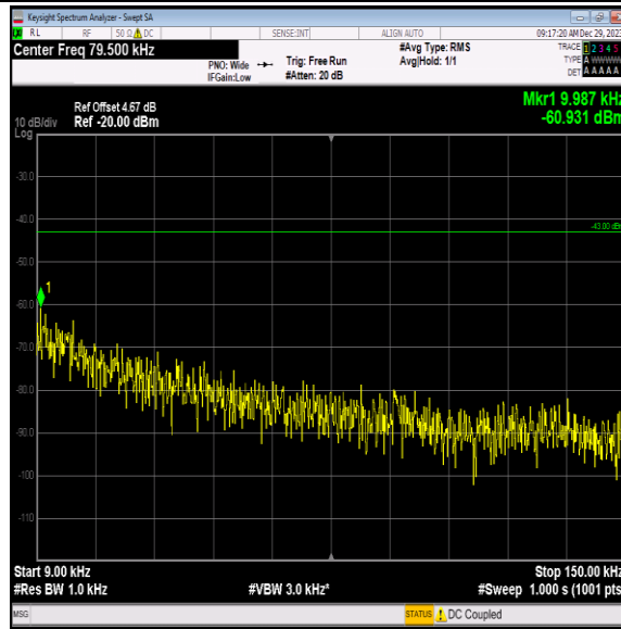
Band4-1513-2-0.009~0.15MHz-PASS
