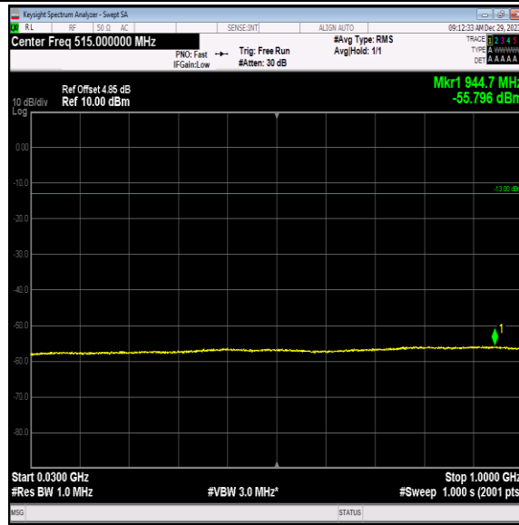
Band4-1413-1-30~1000MHz-PASS
