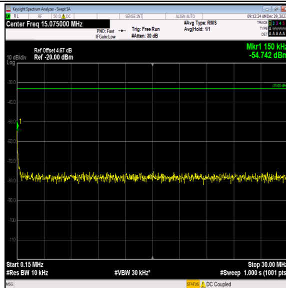
Band4-1413-1-0.15~30MHz-PASS
