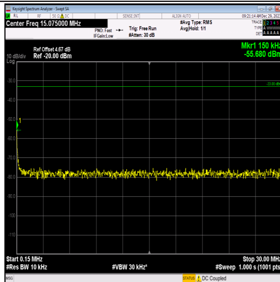
Band4-1513-3-0.15~30MHz-PASS
