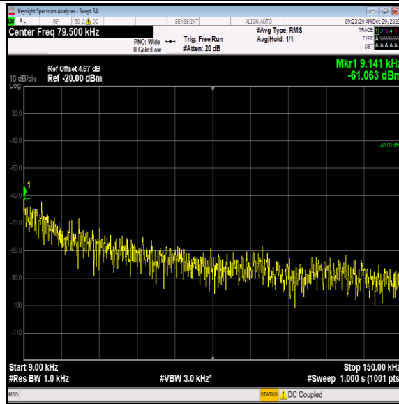
Band4-1413-4-0.009~0.15MHz-PASS
