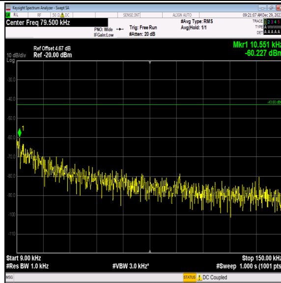
Band4-1513-3-0.009~0.15MHz-PASS
