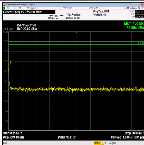
Band4-1513-5-0.15~30MHz-PASS
