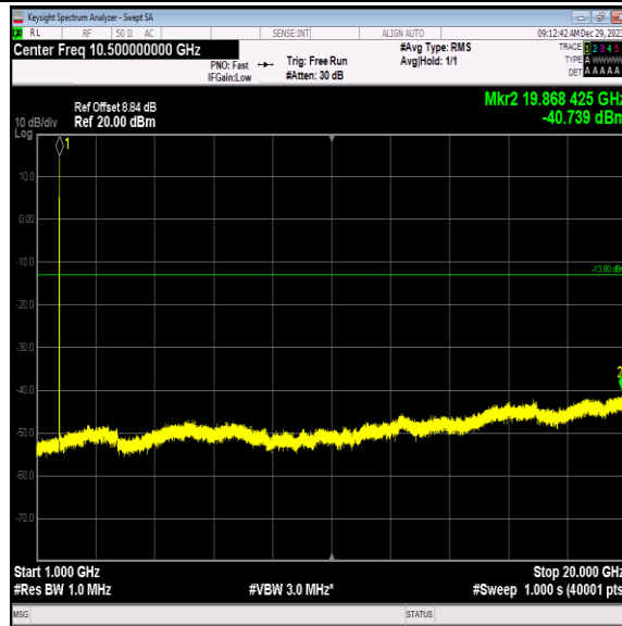
Band4-1413-1-1000~20000MHz-PASS
