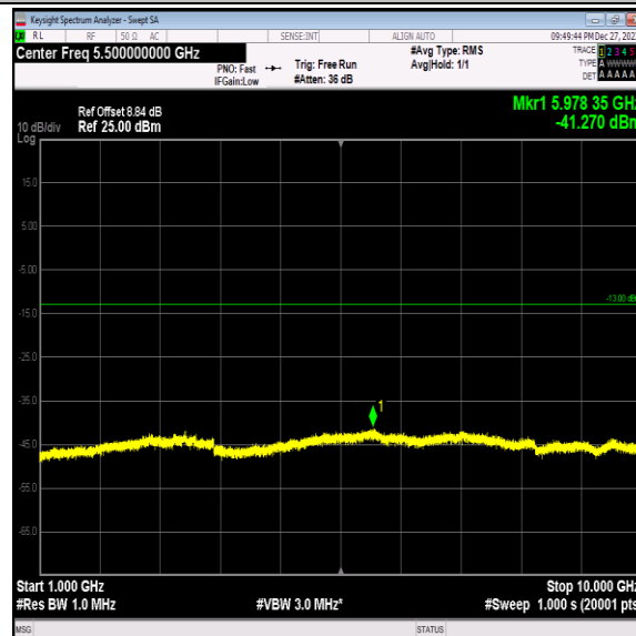
Band5-4132-5-1000~10000MHz-PASS
