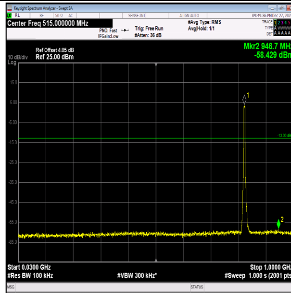
Band5-4132-5-30~1000MHz-PASS
