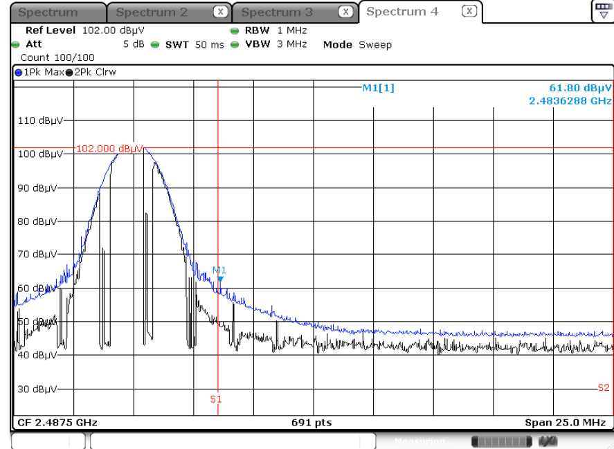
Radiated Restricted Band Edges plot – Average & Peak Result (8DPSK, Ch.78, X-H)
