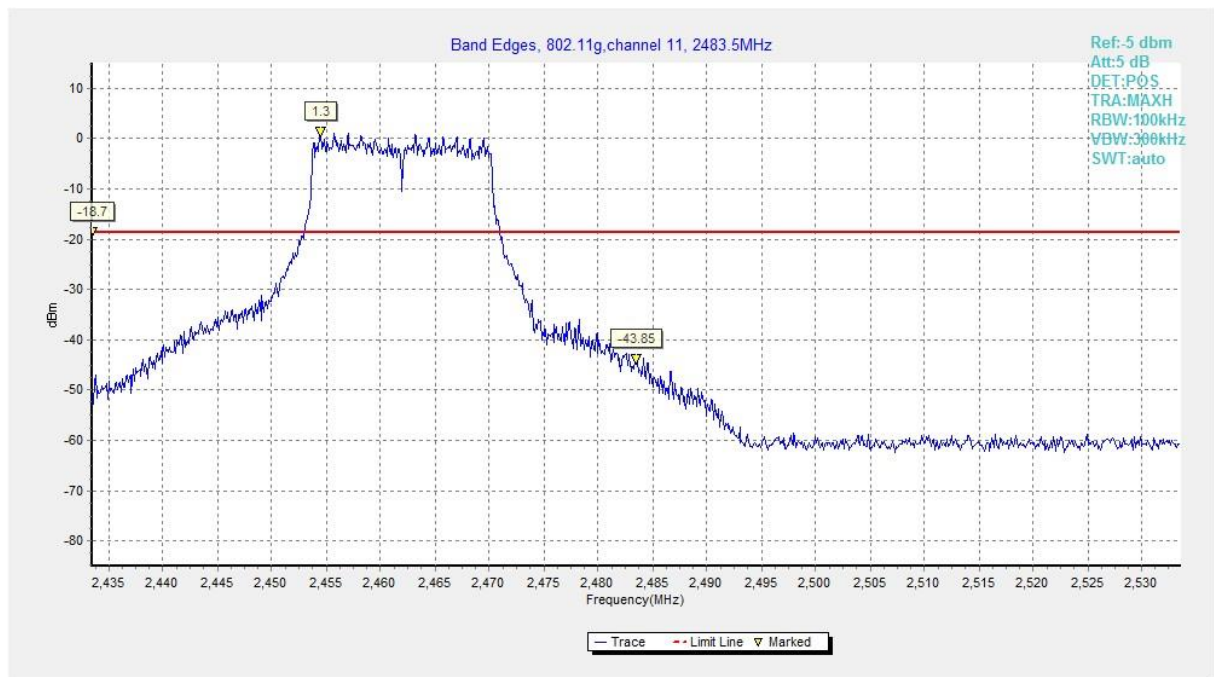
Fig.A.5.5 Band Edges (802.11g, Ch 11)
