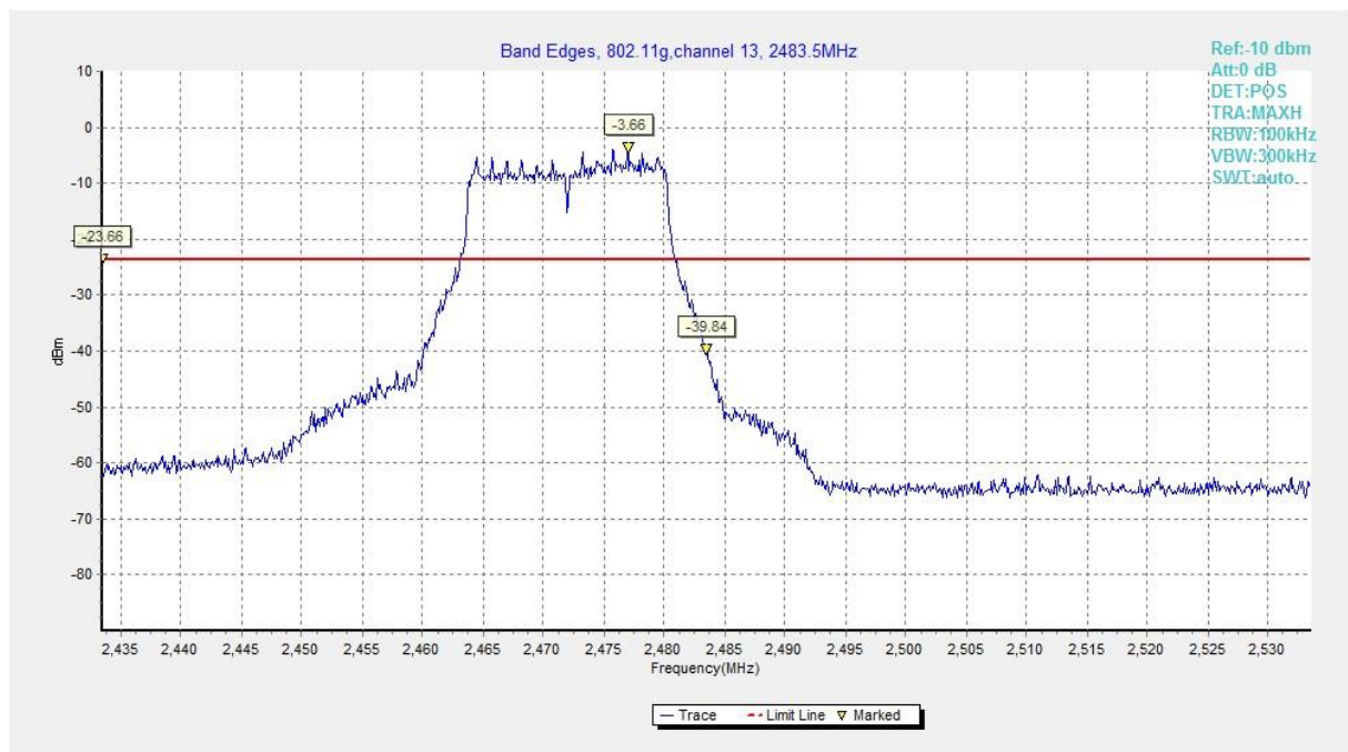
Fig.A.5.6 Band Edges (802.11g, Ch 13)
