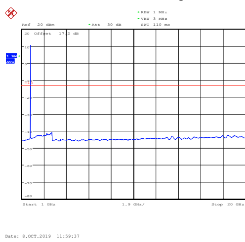
LTE Band 4 1.4MHz CH-High 1GHz~20GHz
