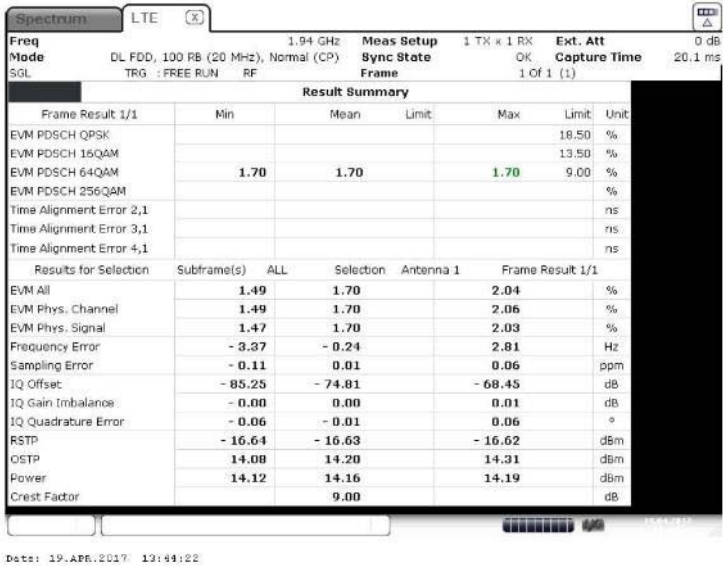
Figure 10 I/Q constellation table with I/Q error – 64QAM (1940.0 MHz) (20MHz Channel BW)
