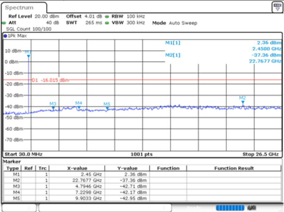
Tx. Spurious NVNT GFSK 2440.705MHz Ant1 Emission
