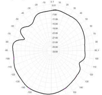
Total(H-XY), Max=-1.81dBi, CrD=11.66
