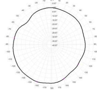
Total(H-XY), Max=-3.13dBi, CrD=7.04
