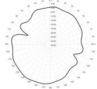
Total(H-XY), Max=-1.94dBi, CrD=16.56
