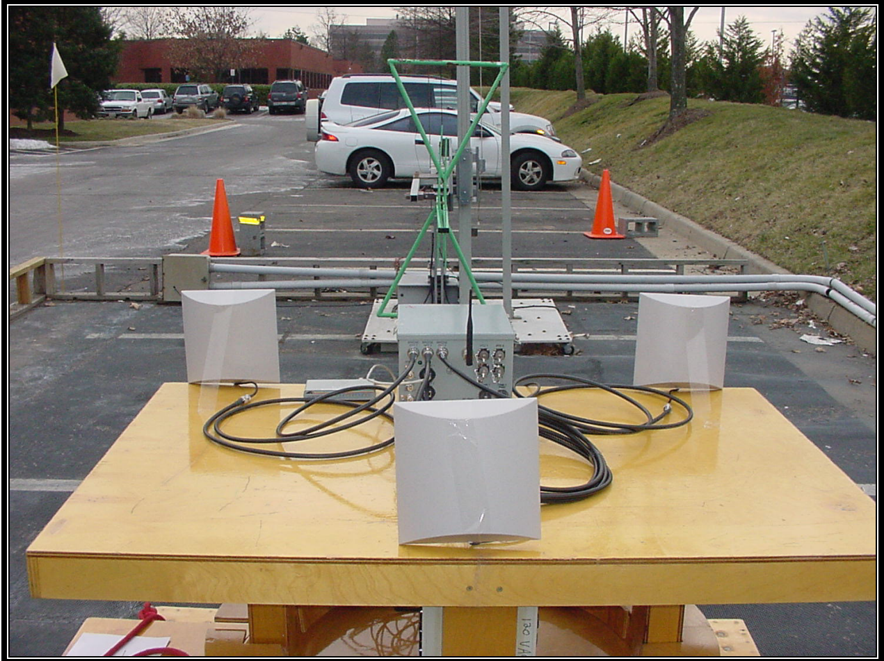
PHOTOGRAPH 2: RADIATED TESTING – REAR VIEW
