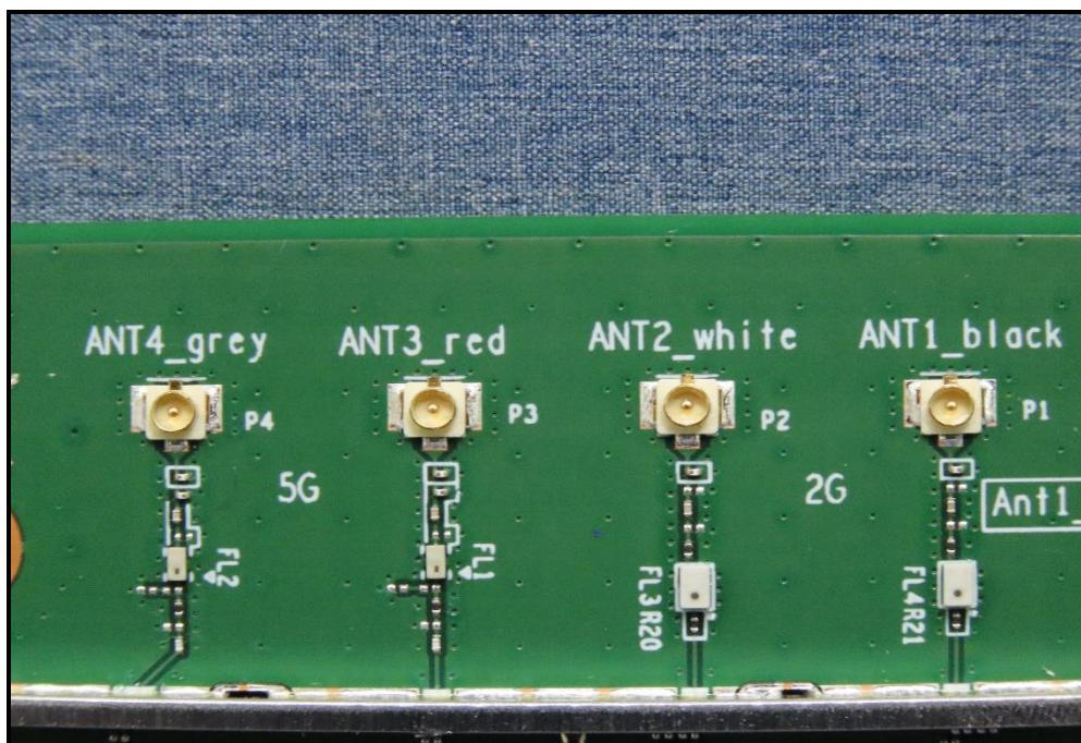
ANT 1 / Model: 290-20509
