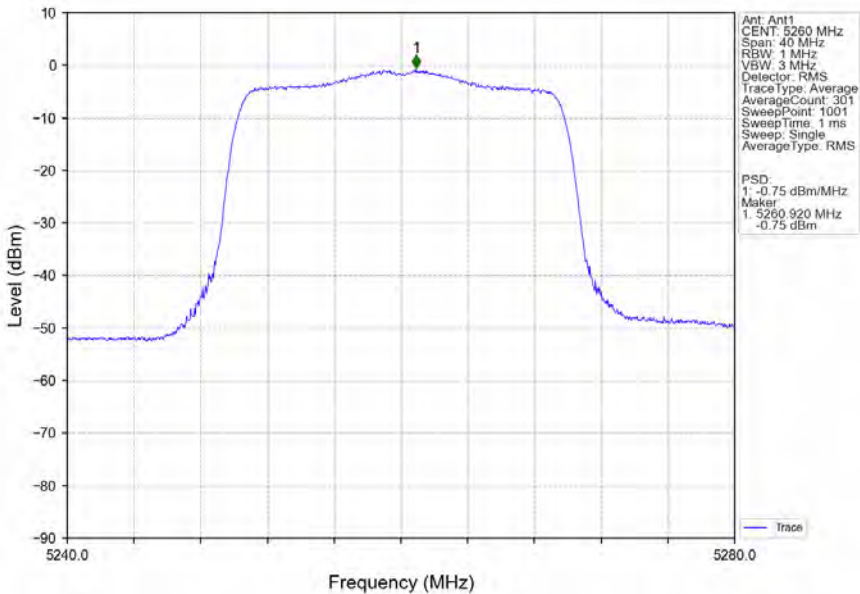
802.11ax(HEW20)_LCH_5260MHz_SU_ / _Ant1_NTNV
