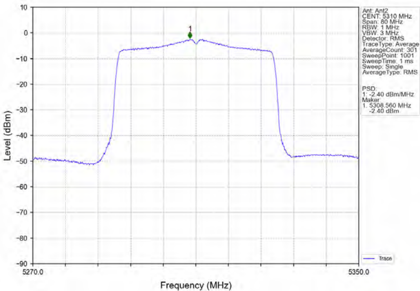
802.11ax(HEW40)_HCH_5310MHz_SU_/_Ant2_NTNV
