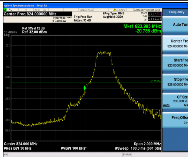
Band26_3MHz_16QAM_20415_1RB#0
