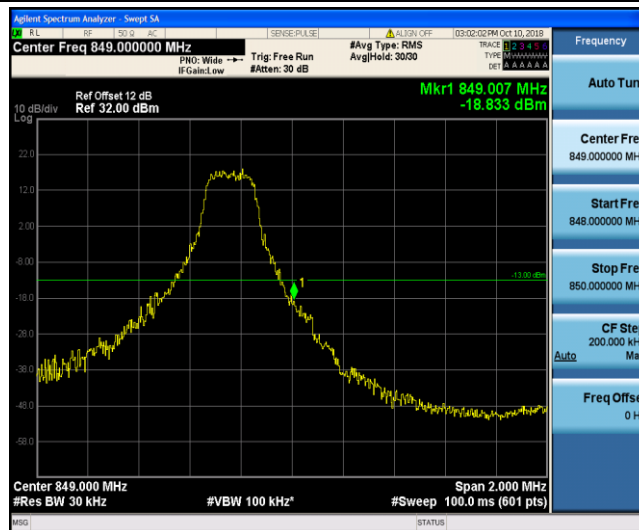
Band26_3MHz_QPSK_20635_1RB#14
