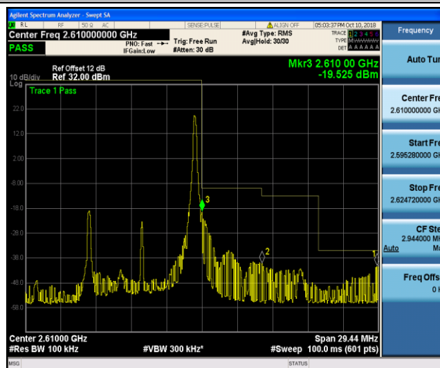
Band41_10MHz_QPSK_40740_1RB#49
