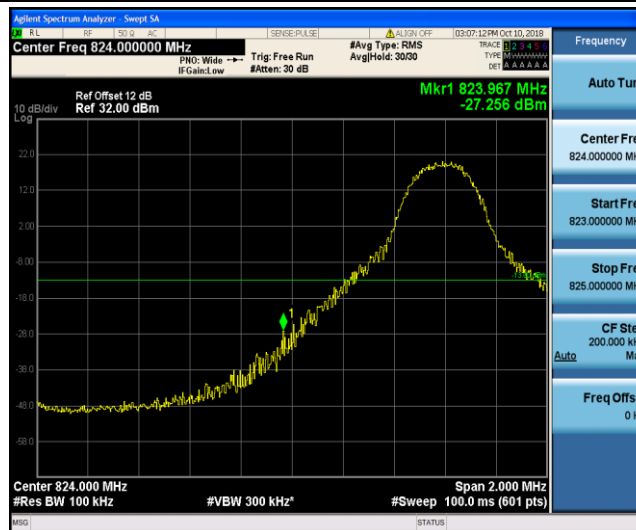
Band26_10MHz_16QAM_20450_1RB#0
