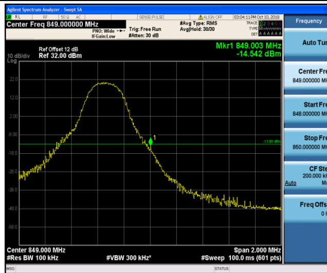
Band26_5MHz_QPSK_20625_1RB#24
