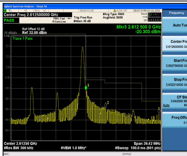
Band41_15MHz_QPSK_40740_1RB#74
