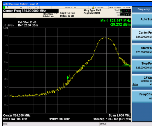
Band26_10MHz_QPSK_20450_1RB#0
