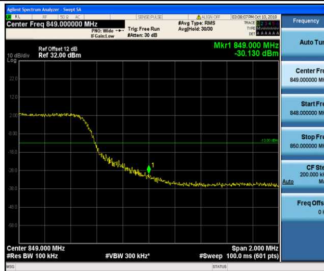
Band26_10MHz_QPSK_20600_50RB#0
