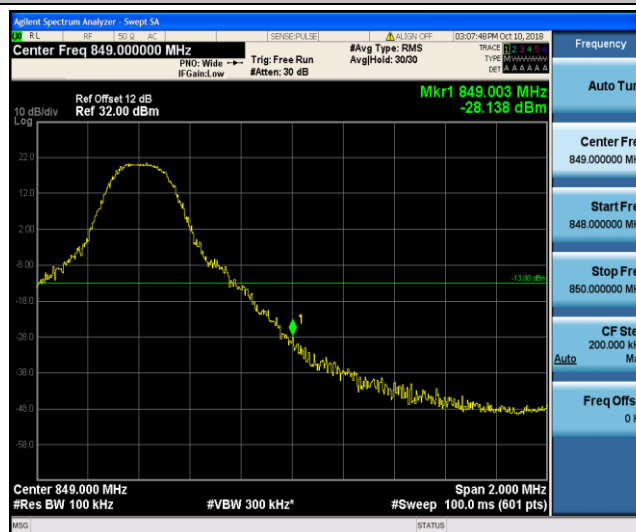
Band26_10MHz_QPSK_20600_1RB#49
