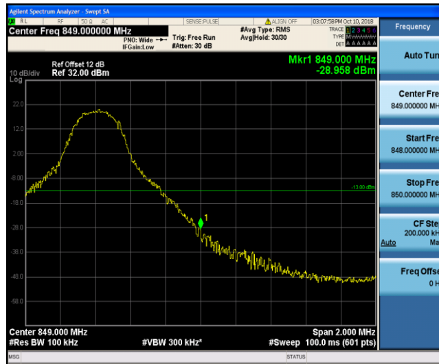
Band26_10MHz_16QAM_20600_1RB#49
