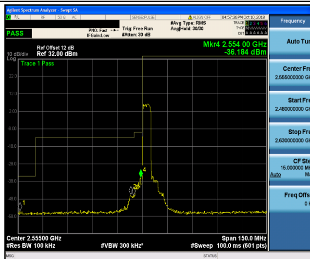
Band41_5MHz_QPSK_40265_25RB#0
