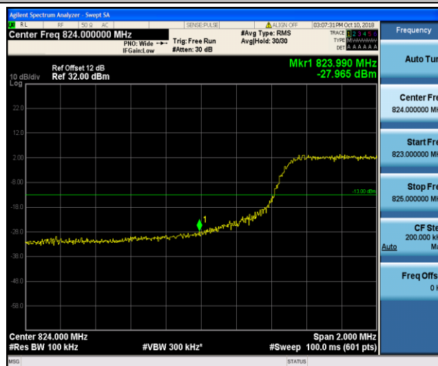
Band26_10MHz_16QAM_20450_50RB#0
