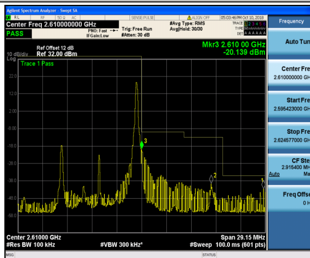
Band41_10MHz_16QAM_40740_1RB#49
