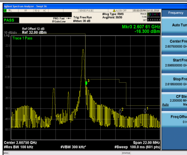
Band41_5MHz_16QAM_40740_1RB#24
