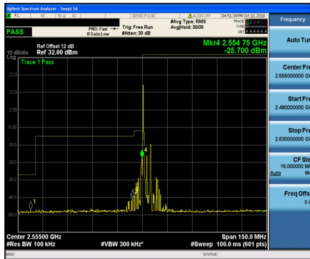
Band41_5MHz_QPSK_40265_1RB#0
