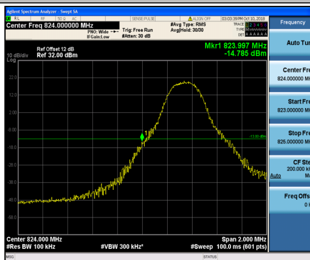
Band26_5MHz_16QAM_20425_1RB#0
