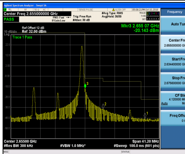
Band41_15MHz_QPSK_41165_1RB#74
