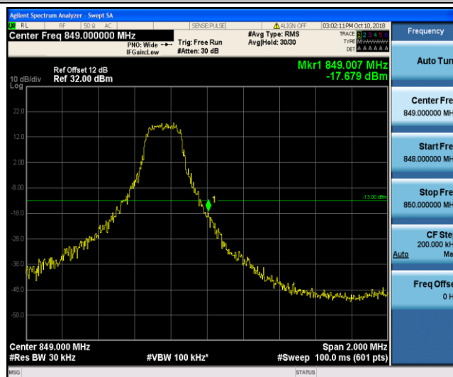
Band26_3MHz_16QAM_20635_1RB#14
