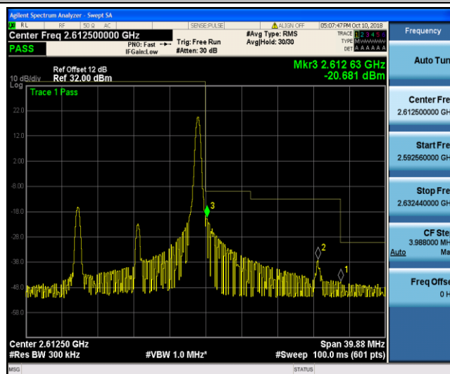
Band41_15MHz_16QAM_40740_1RB#74
