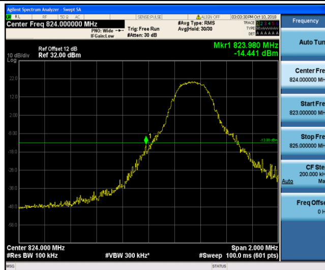
Band26_5MHz_QPSK_20425_1RB#0
