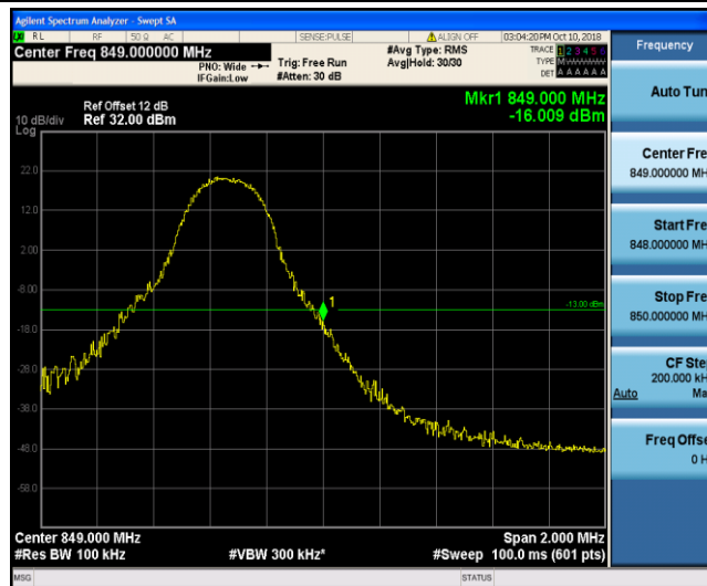
Band26_5MHz_16QAM_20625_1RB#24
