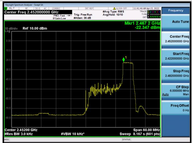
802.11ax-40 MHz(RU52) CHANNEL 9
