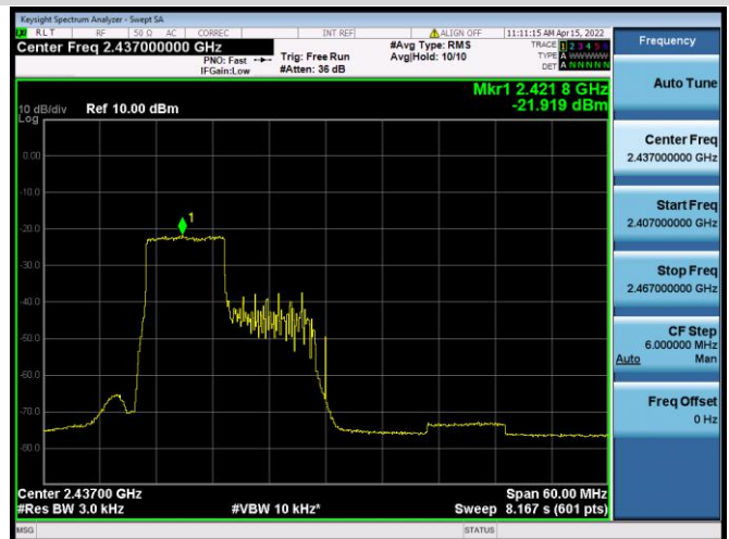
802.11ax-40 MHz(RU106) CHANNEL 6
