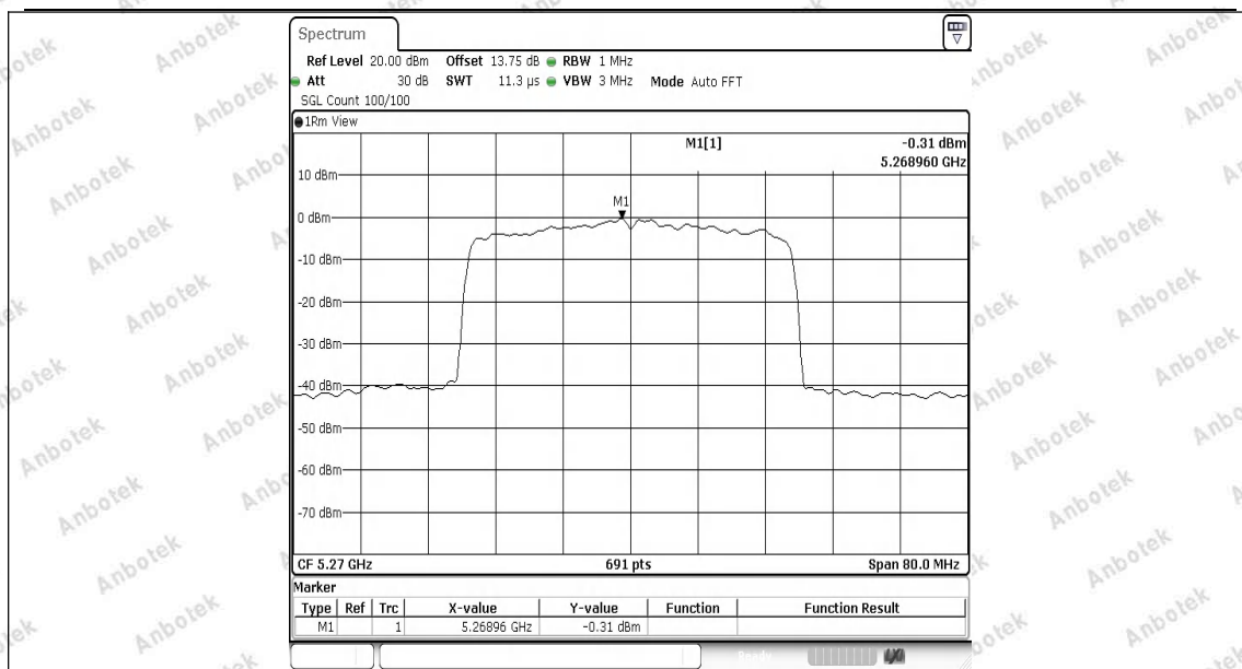
11AX40SISO-Ant1-5270-PASS
