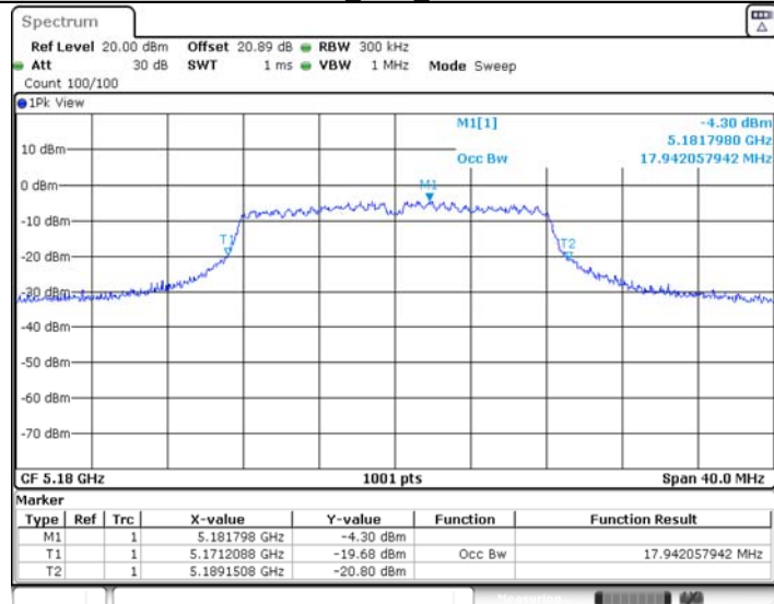
11A_Ant2_5180
