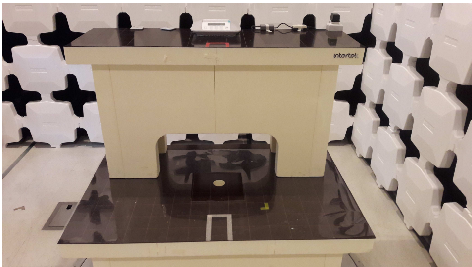
Radiated Emission
