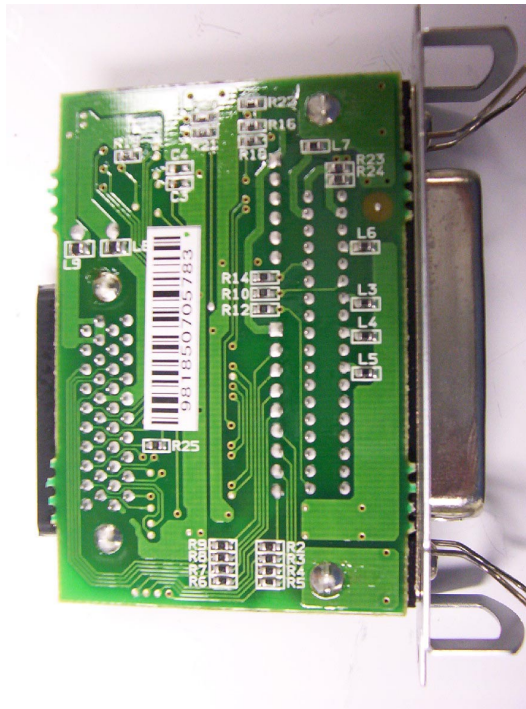
Printer I/O PCB bottom
