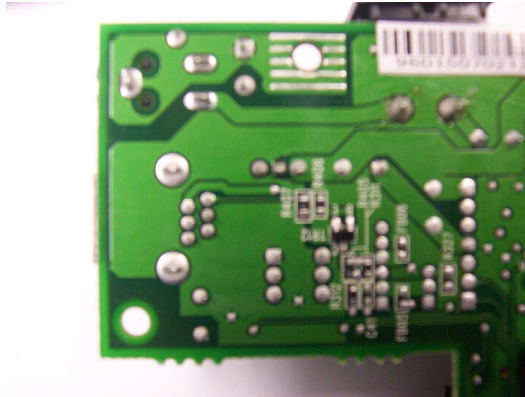
Printer PCB bottom 3
