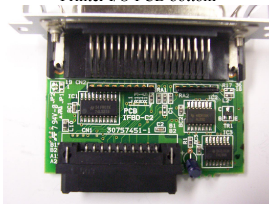
Printer I/O PCB Top
