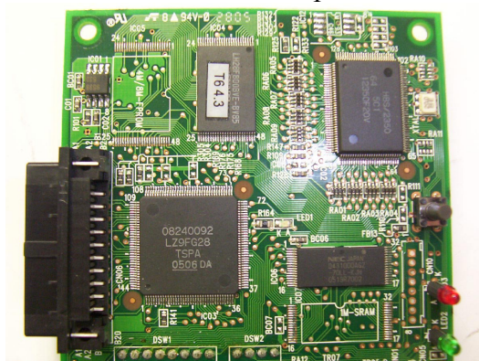
Printer PCB top 1
