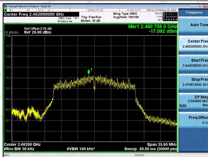
11AX20SISO-Ant1-2462-PASS
