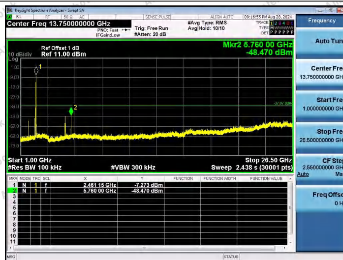
11AX20SISO-Ant1-2462-1000~26500-PASS
