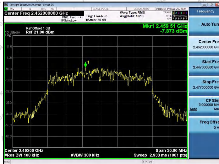
11AX20SISO-Ant1-2462-0~Reference-PASS
