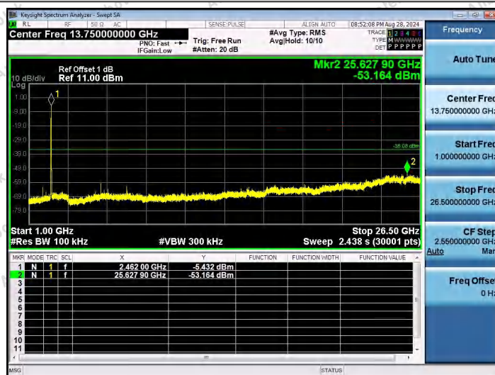
11B-Ant1-2462-1000~26500-PASS
