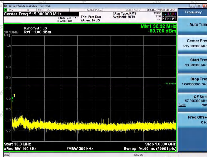
11B-Ant1-2462-30~1000-PASS
