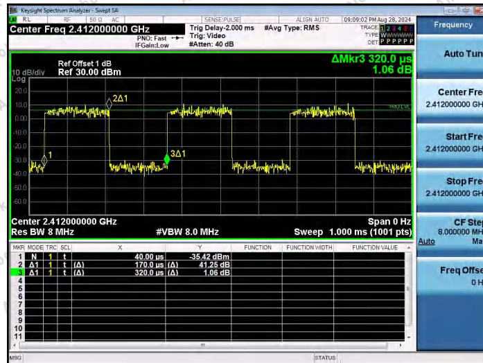
NTNV-11AX20SISO-Ant1-2412
