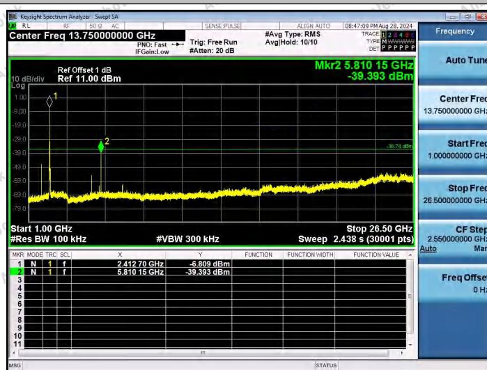
11G-Ant1-2412-1000~26500-PASS
