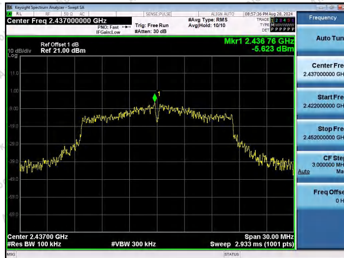
11G-Ant1-2437-0~Reference-PASS
