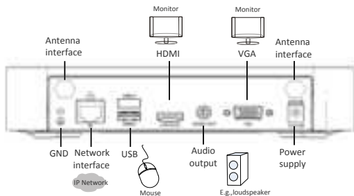
Figure 4-1 NVR Interfaces
