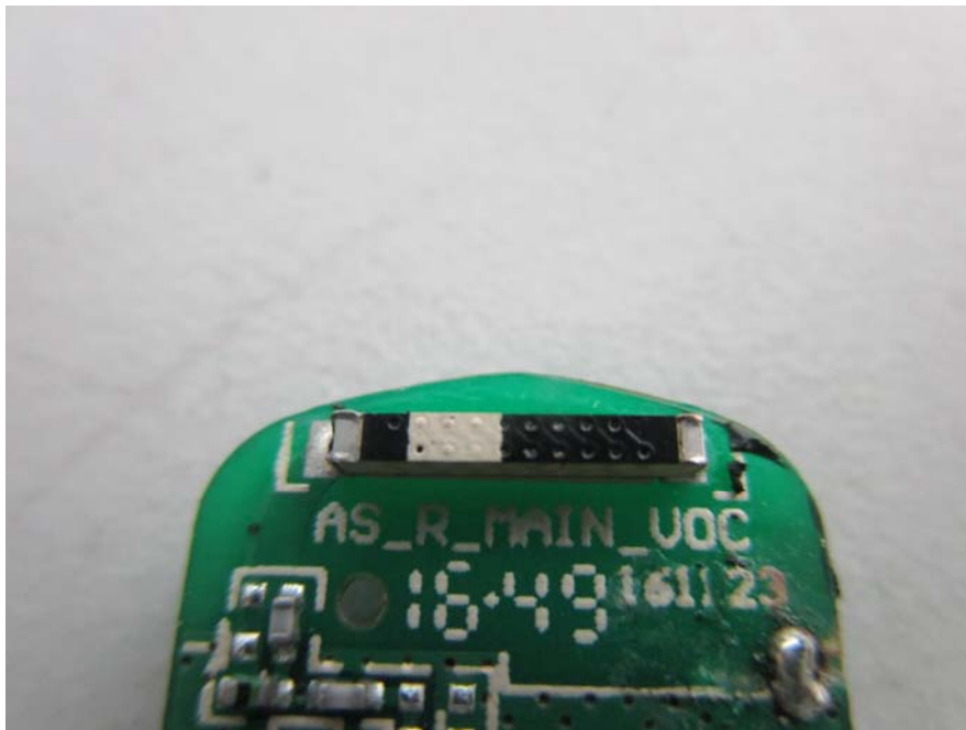
EUT – Right Antenna View
