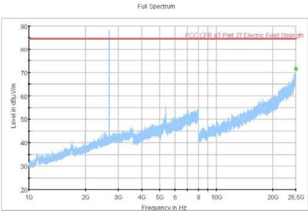
Figure 270 Radiated Emission 1 GHz – 26.5 GHz (2680 MHz) (20MHz Channel BW)
