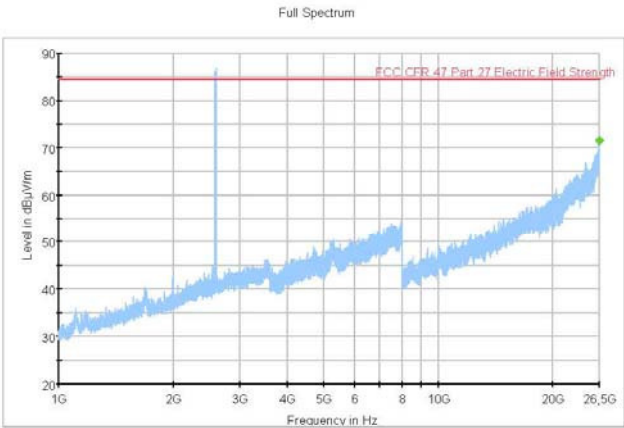
Figure 269 Radiated Emission 1 GHz – 26.5 GHz (2593 MHz) (20MHz Channel BW)
