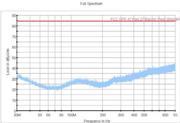
Figure 271 Radiated Emission 30 MHz – 1 GHz (2506 / 2526 MHz) (20MHz Channel BW)
