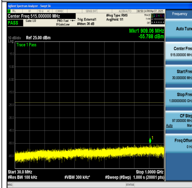
NTNV-n77(3450-3550)-PC2-30-100-H-DFT-BPSK- Edge_1RB_Left-30-1000-PASS
