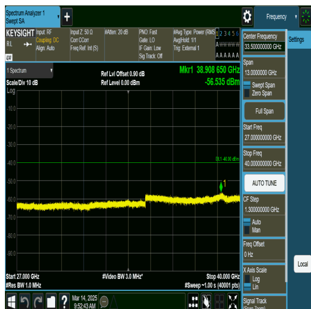
NTNV-n77(3450-3550)-PC2-30-100-H-DFT-BPSK- Edge_1RB_Left-27000-40000-PASS
