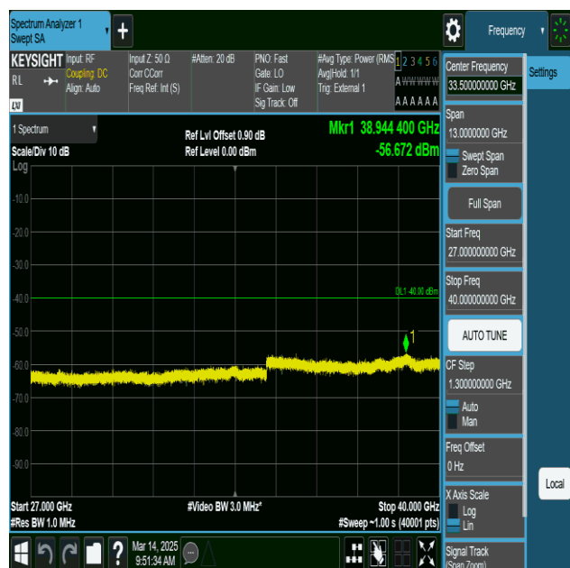
NTNV-n77(3450-3550)-PC2-30-100-L-CP-QPSK- Edge_1RB_Left-27000-40000-PASS
