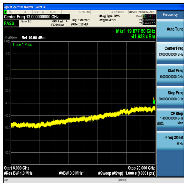
NTNV-n77(3450-3550)-PC2-30-100-L-CP-QPSK- Edge_1RB_Left-6000-20000-PASS
