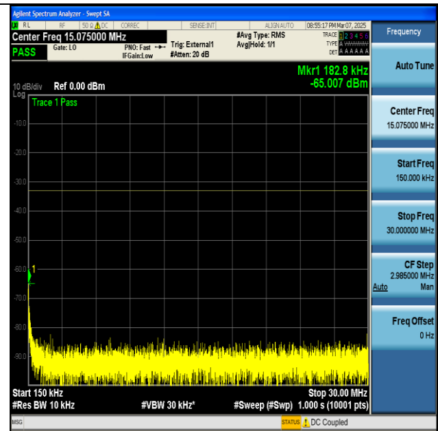
NTNV-n77(3450-3550)-PC2-30-100-M-CP-QPSK- Edge_1RB_Left-0.15-30-PASS
