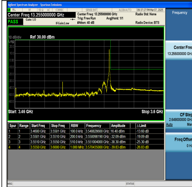
NTNV-n77(3450-3550)-PC2-30-90-H-CP-QPSK- Edge_1RB_Right-PASS
