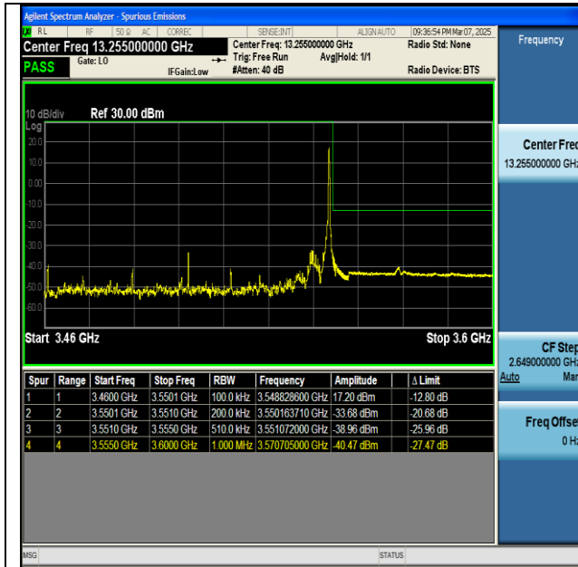
NTNV-n77(3450-3550)-PC2-30-90-H-DFT-BPSK- Edge_1RB_Right-PASS
