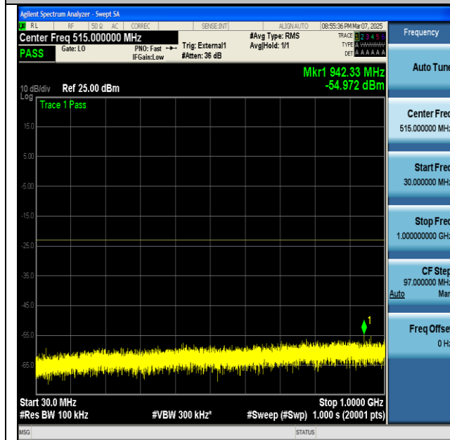
NTNV-n77(3450-3550)-PC2-30-100-M-CP-QPSK- Edge_1RB_Left-30-1000-PASS
