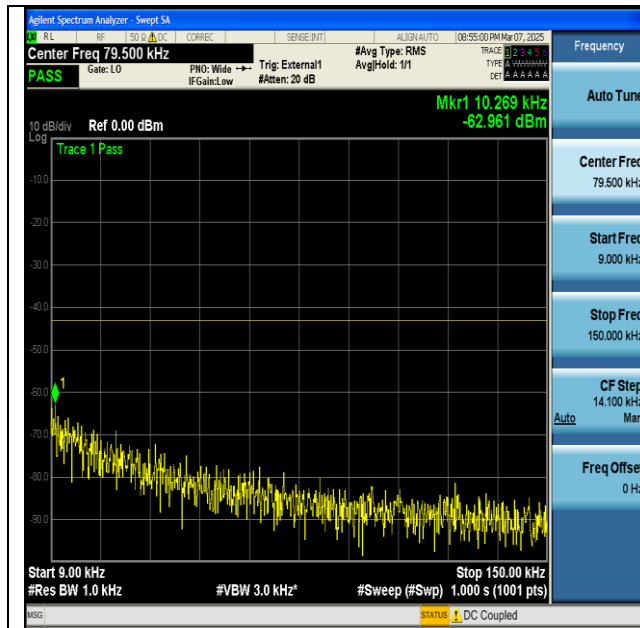
NTNV-n77(3450-3550)-PC2-30-100-M-CP-QPSK- Edge_1RB_Left-0.009-0.15-PASS
