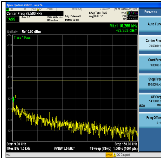
NTNV-n77(3450-3550)-PC2-30-100-H-DFT-BPSK- Edge_1RB_Left-0.009-0.15-PASS
