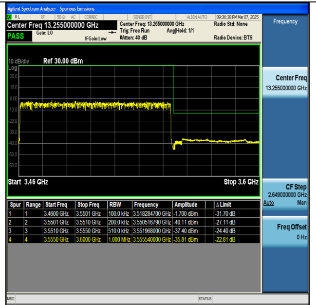
NTNV-n77(3450-3550)-PC2-30-90-H-DFT-BPSK- Outer_Full-PASS
