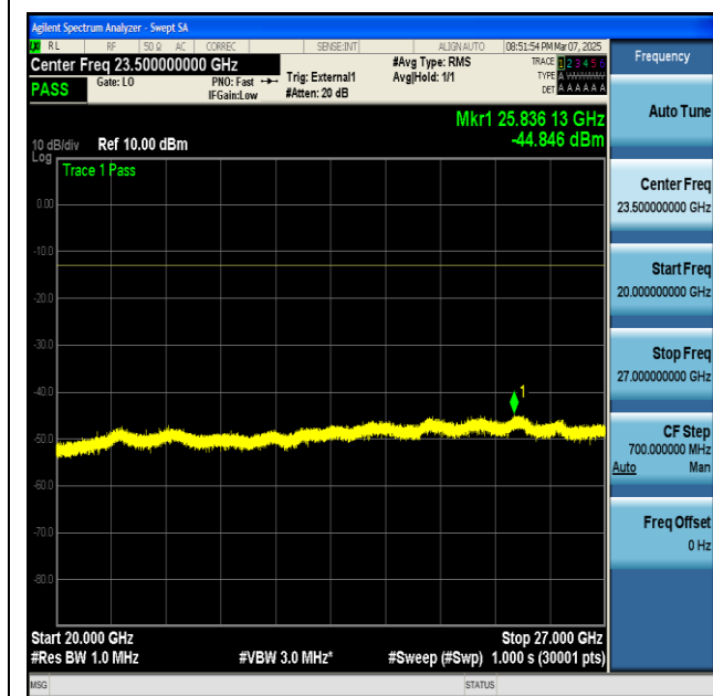
NTNV-n77(3450-3550)-PC2-30-100-L-CP-QPSK- Edge_1RB_Left-20000-27000-PASS
