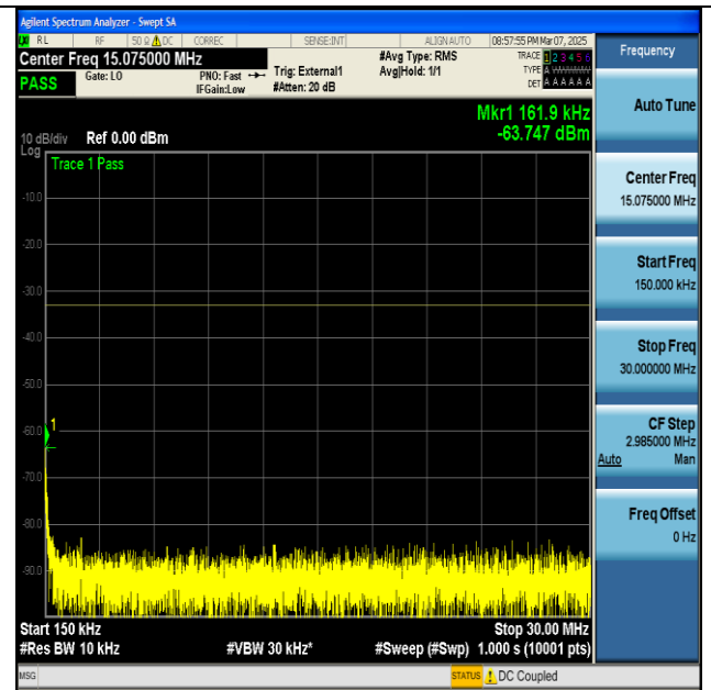
NTNV-n77(3450-3550)-PC2-30-100-H-DFT-BPSK- Edge_1RB_Left-0.15-30-PASS
