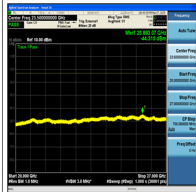
NTNV-n77(3450-3550)-PC2-30-100-L-DFT-BPSK- Edge_1RB_Left-20000-27000-PASS
