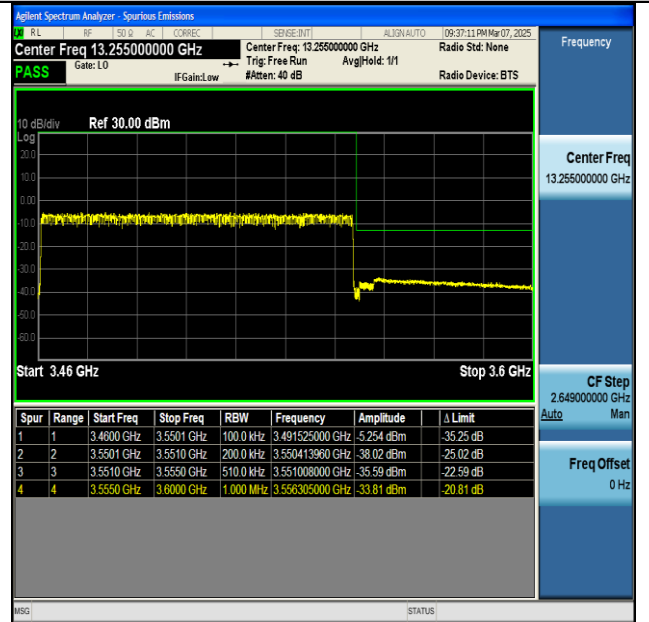
NTNV-n77(3450-3550)-PC2-30-90-H-CP-QPSK- Outer_Full-PASS
