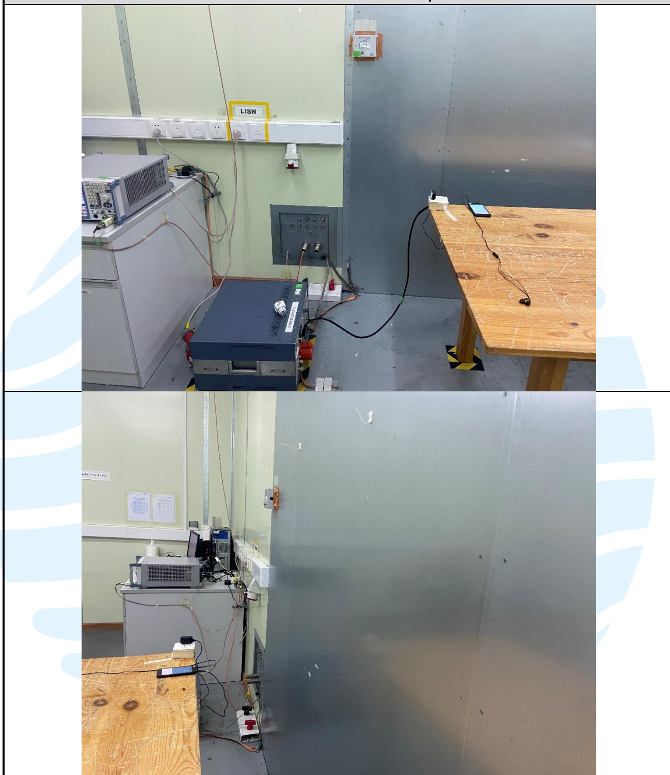
Conducted Emission Test Setup-3
