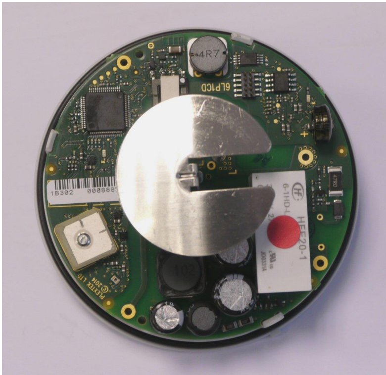
Assembled internal view 2:
