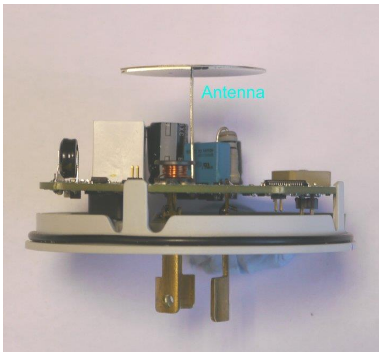
Assembled internal view 2:
