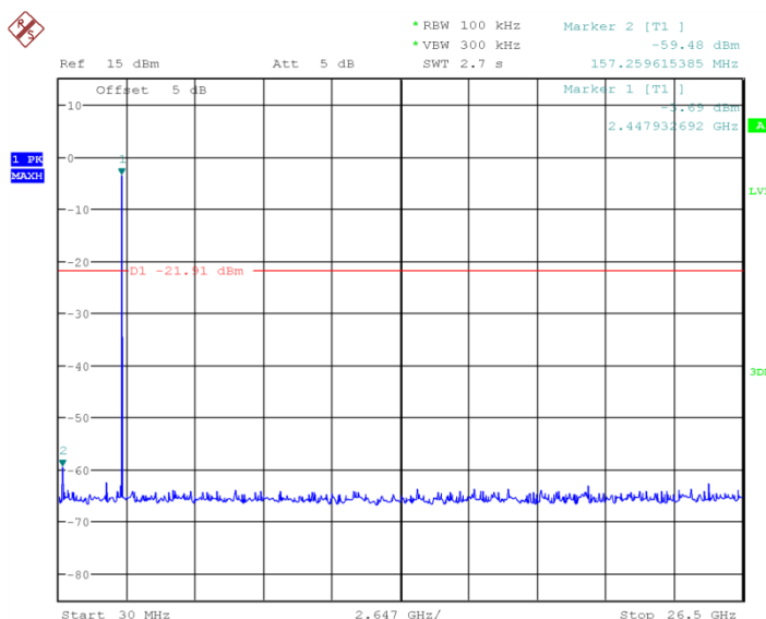
Fig.17 Conducted spurious emission: Ch39, 30MHz~26GHz
