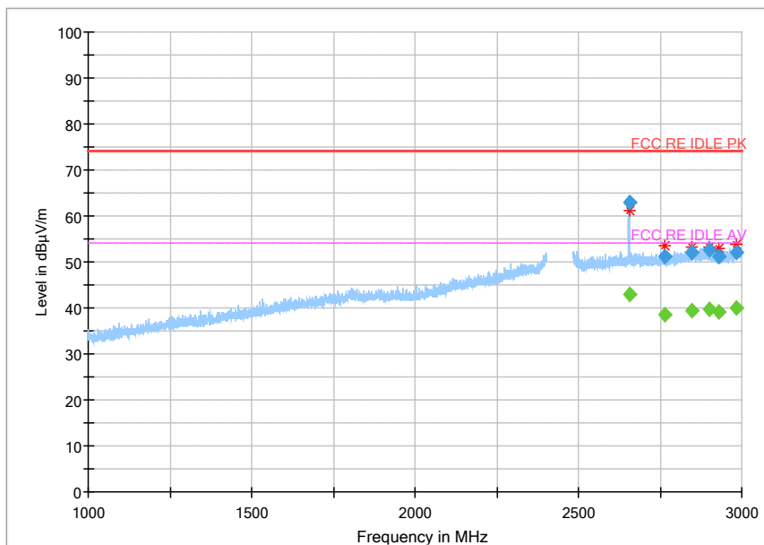
Fig.25 Radiated emission: Ch39, 1GHz~3GHz
