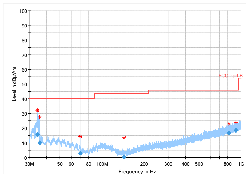
Fig.21 Radiated emission: Ch0, 30MHz~1GHz
