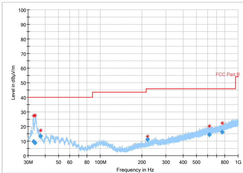
Fig.24 Radiated emission: Ch39, 30MHz~1GHz
