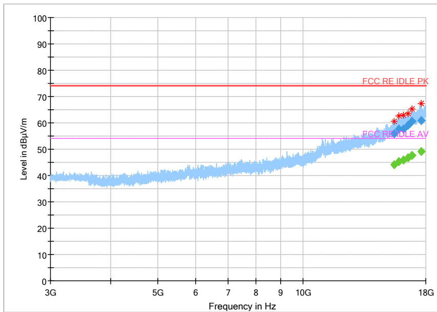
Fig.20 Radiated emission: Ch0, 3GHz~18GHz
