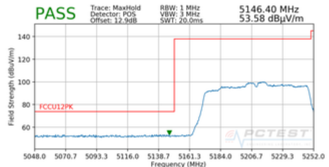
Plot 7-89. Radiated Lower Band Edge Plot MIMO (Peak – UNII Band 1)
