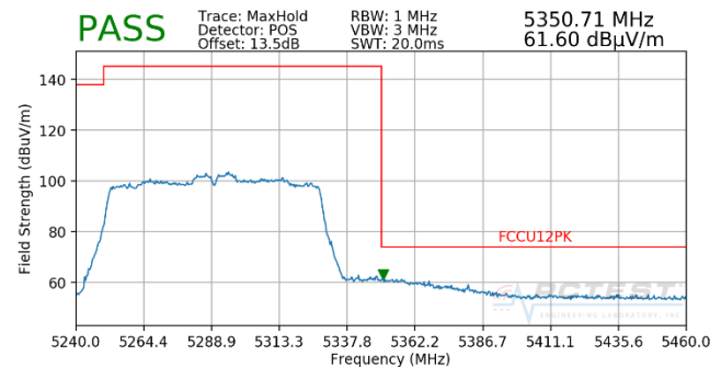
Plot 7-91. Radiated Upper Band Edge Plot MIMO (Peak – UNII Band 2A)
