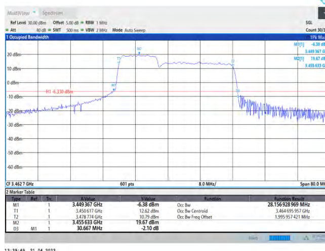
42-42-10MHz-20MHz-QPSK-QPSK-42496-42640-50RB#0-100RB#0
