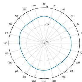
Total_Polar_H_5.55GHz
