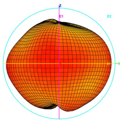
Total_3D_E2_5.55GHz
