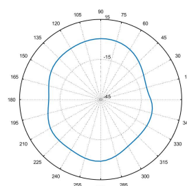
Total_Polar_E2_5.55GHz
