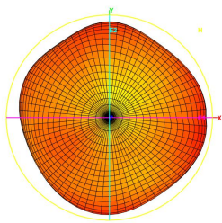
Total_3D_H_5.55GHz
