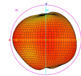
Total_3D_E1_5.55GHz
