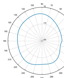
Total_3D_H_5.55GHz
