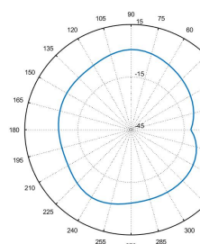
Total_Polar_E1_5.55GHz
