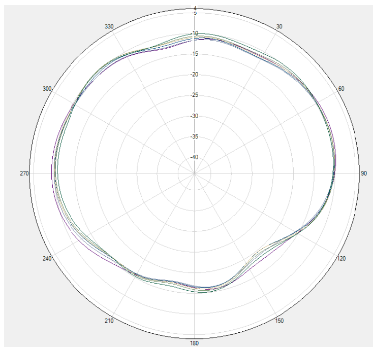
LTE B40 \Theta = 90^\circ
