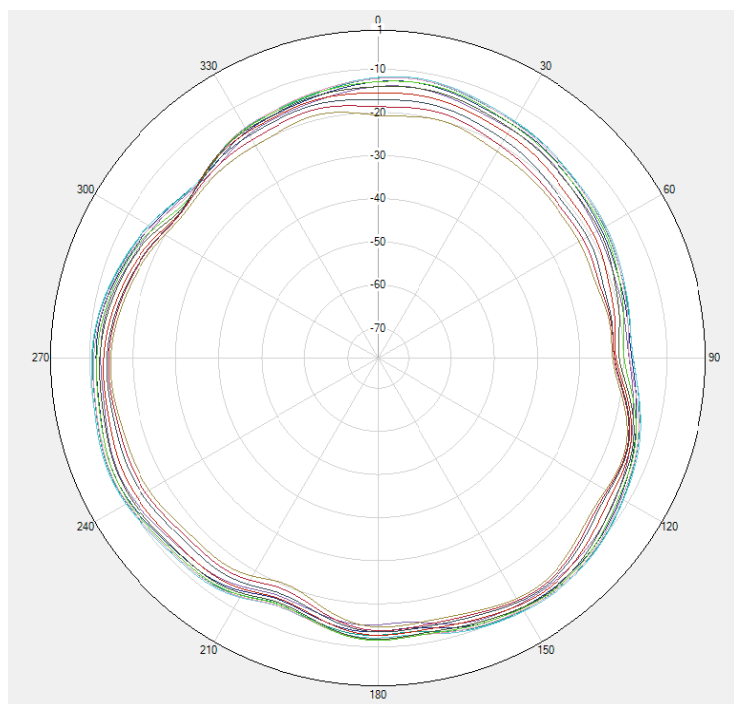
GSM900 / WCDMA B8 / LTE B8 \Phi = 0^\circ
