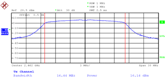
Mode: 802.11g channel 11
