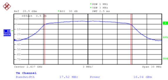
Mode: 802.11n HT20 channel 6
