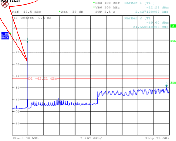
Mode: 802.11b channel 6
