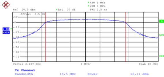
Mode: 802.11g channel 6
