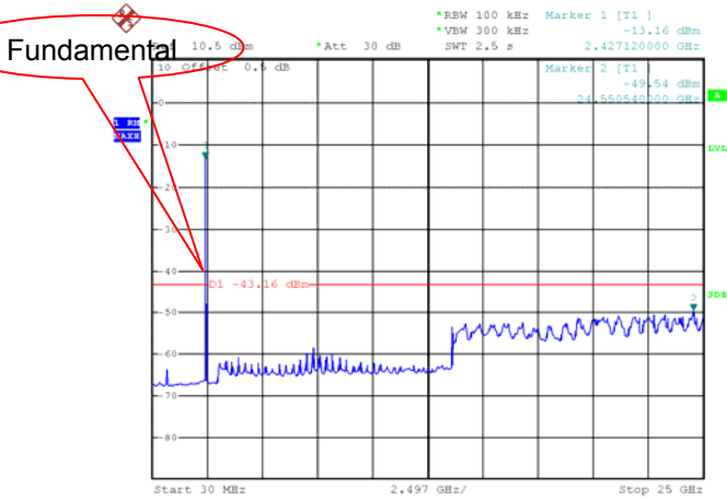
Mode: 802.11 n HT20 channel 6
