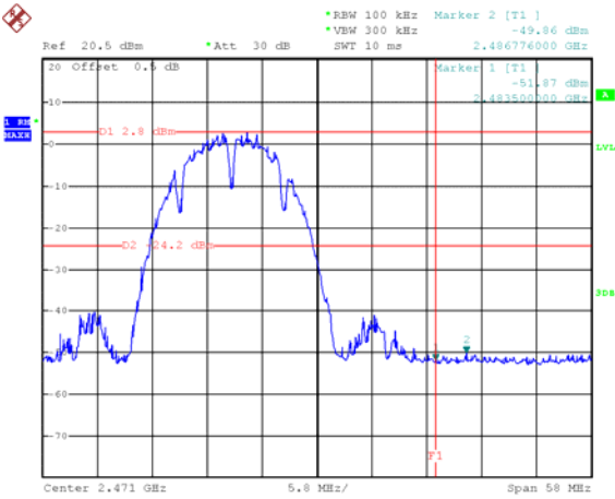
802.11b: Band edge-right side
