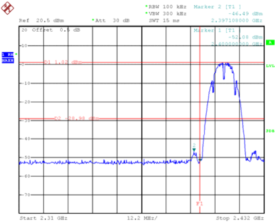
802.11b: Band edge-left side
