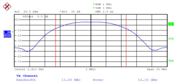
Mode: 802.11b channel 1
