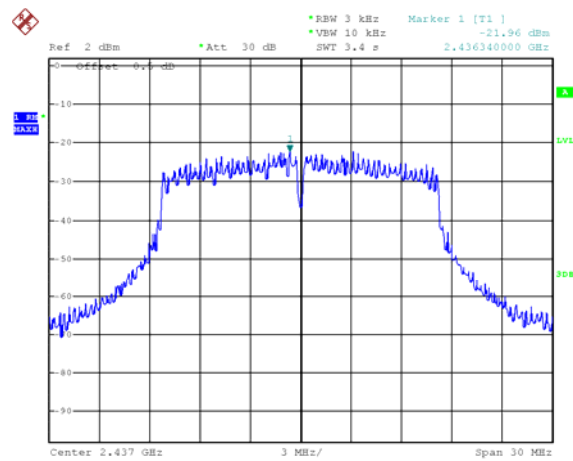
Mode: 802.11g channel 6
