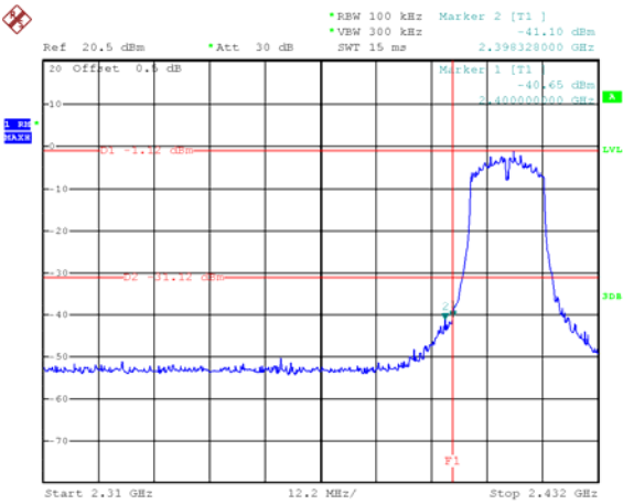
802.11g: Band edge-left side
