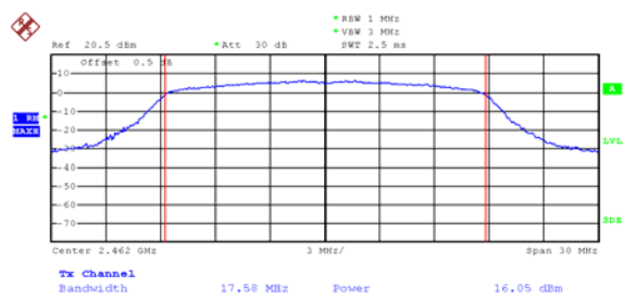
Mode: 802.11n HT20 channel 11
