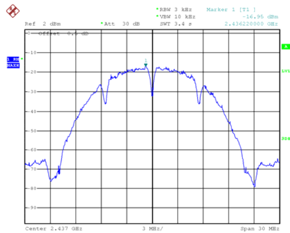
Mode: 802.11b channel 6
