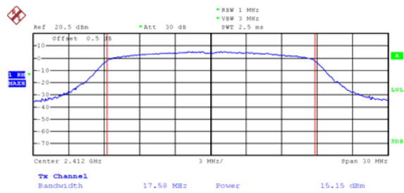
Mode: 802.11n HT20 channel 1
