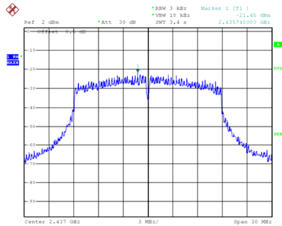
Mode: 802.11n HT20 channel 6
