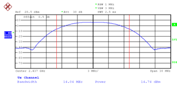
Mode: 802.11b channel 6
