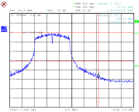
802.11g: Band edge-right side
