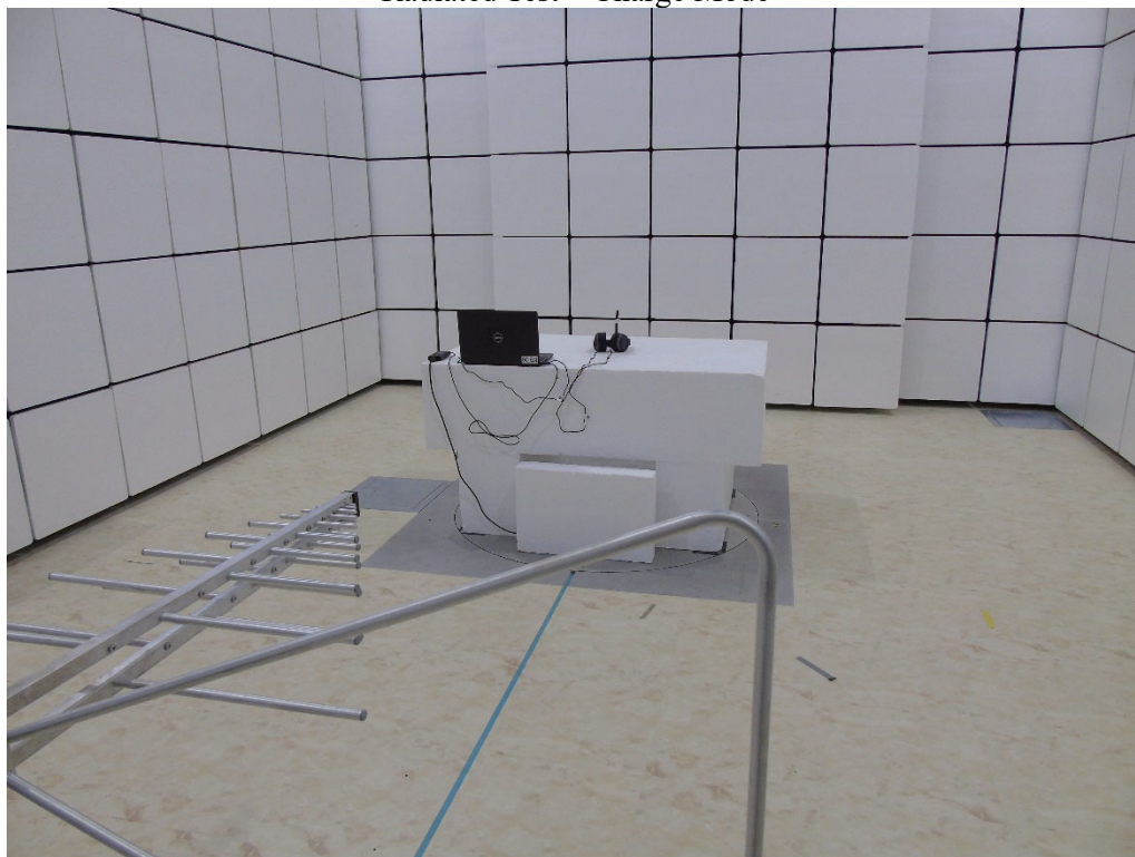
Radiated Test – Charge Mode
