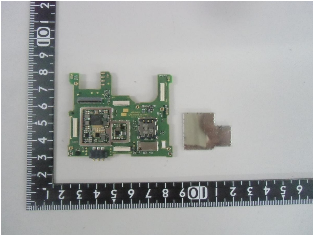
Main PCB Rear (without shield)
