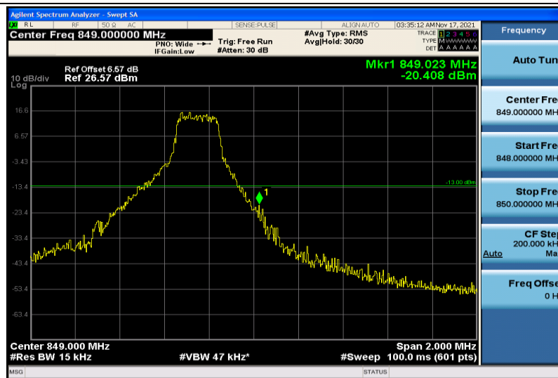
Band5-1.4MHz-16QAM-20643-1RB#5
