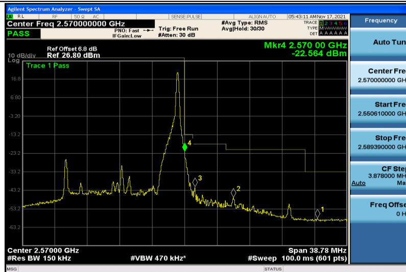
Band7-15MHz-QPSK-21375-1RB#74
