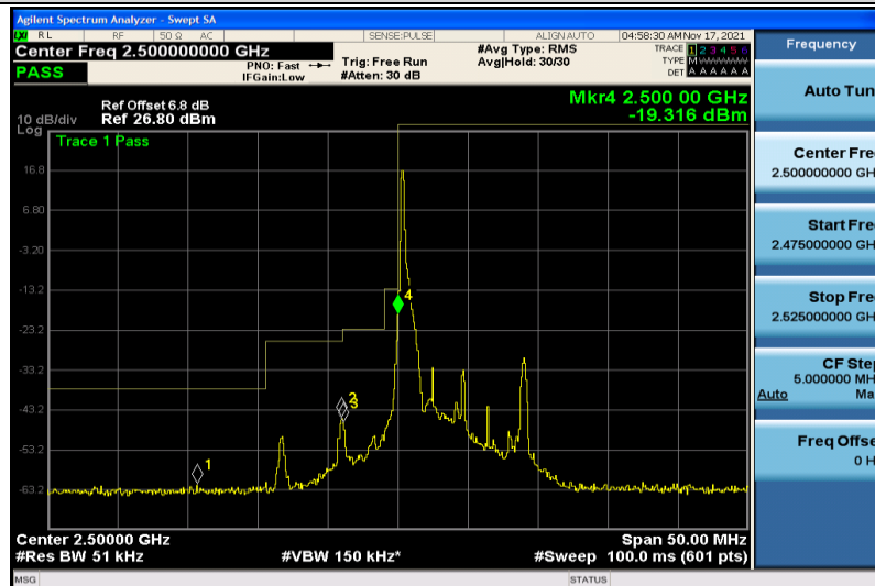
Band7-5MHz-QPSK-20775-1RB#0
