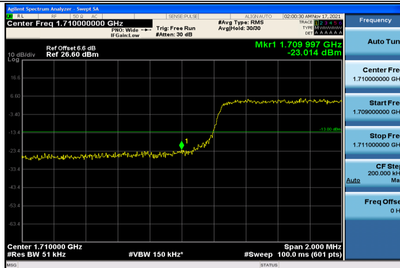
Band4-5MHz-QPSK-19975-25RB#0
