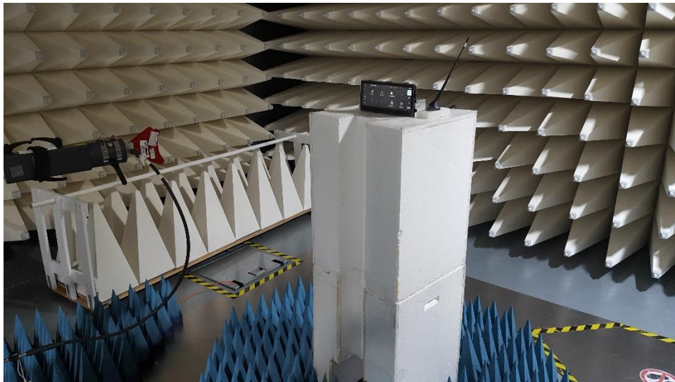
Figure C6. Radiated emission Setup 3
