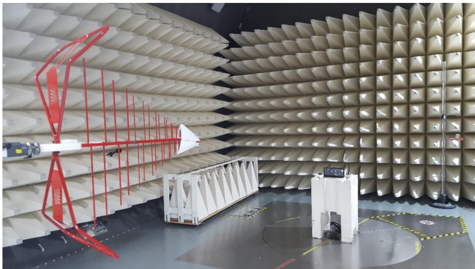
Figure C4. Radiated emission Setup 1
