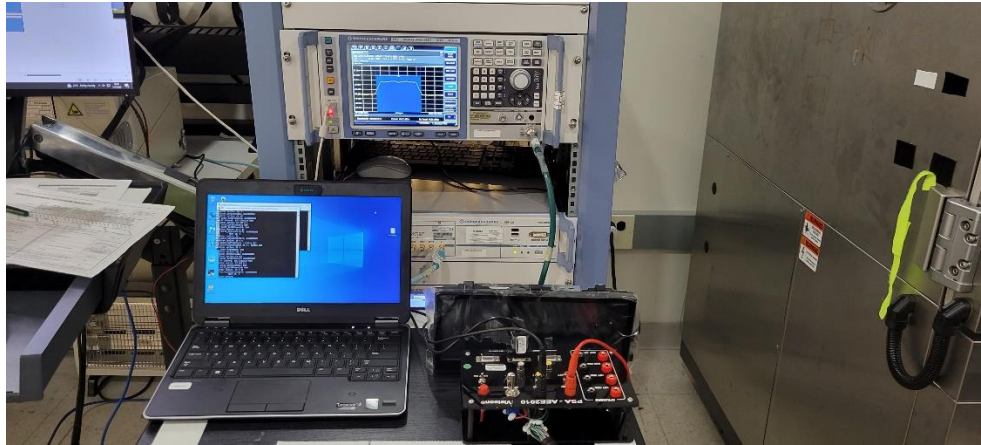
Figure C3. Conducted test setup
