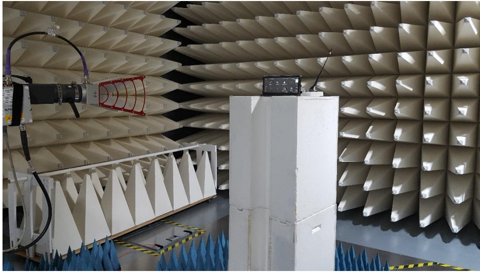
Figure C5. Radiated emission Setup 2
