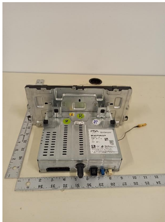
Figure C2. DUT rear view
