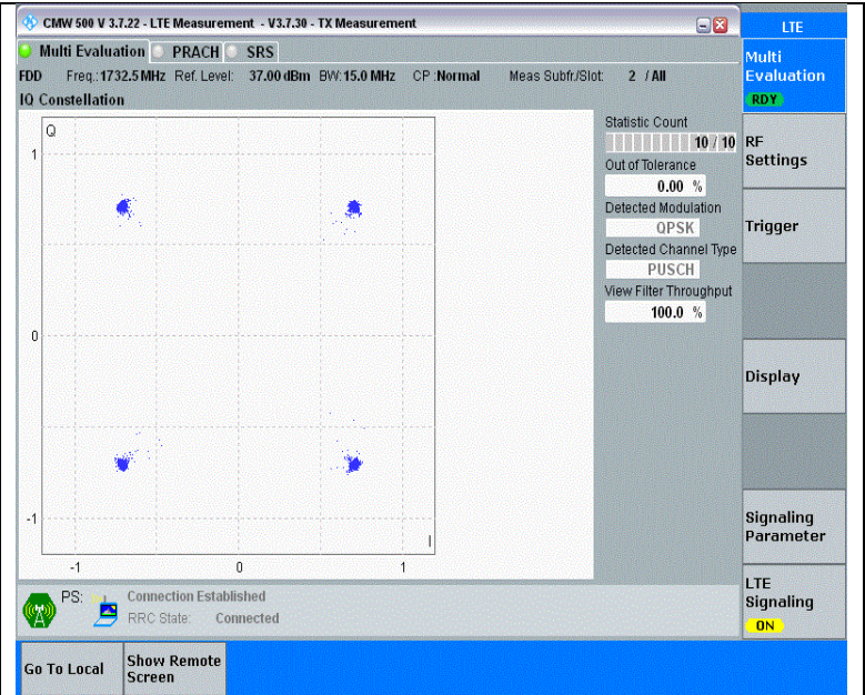
Band4-15MHz-QPSK-20175-75RB#0-PASS
