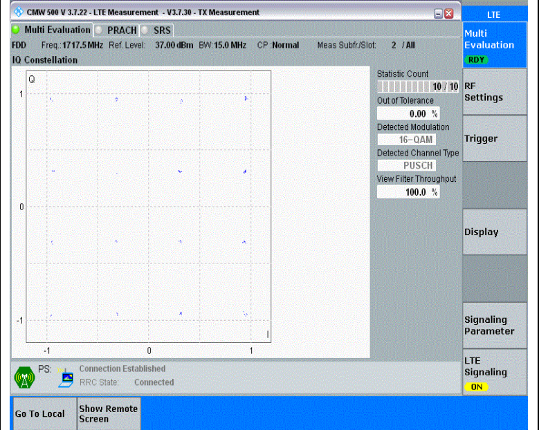
Band4-15MHz-16QAM-20025-1RB#0-PASS
