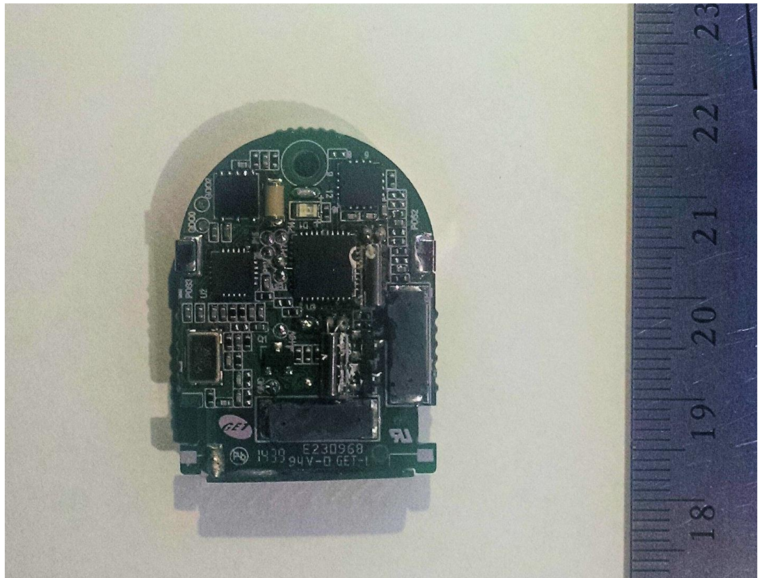
7.3 PCB Component Side View
