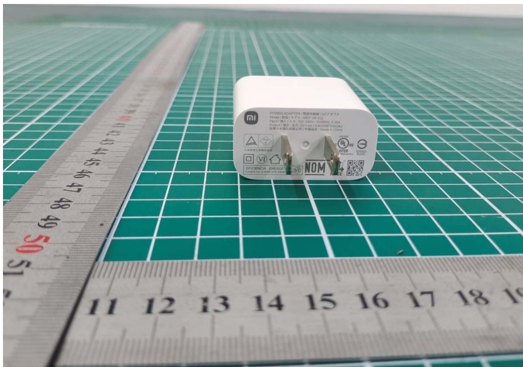
b: Adapter
