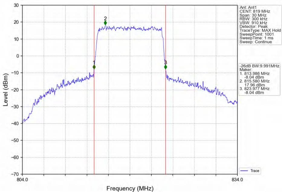
Band26a_10MHz_16QAM_MCH_819MHz_RB_50_0_NTNV
