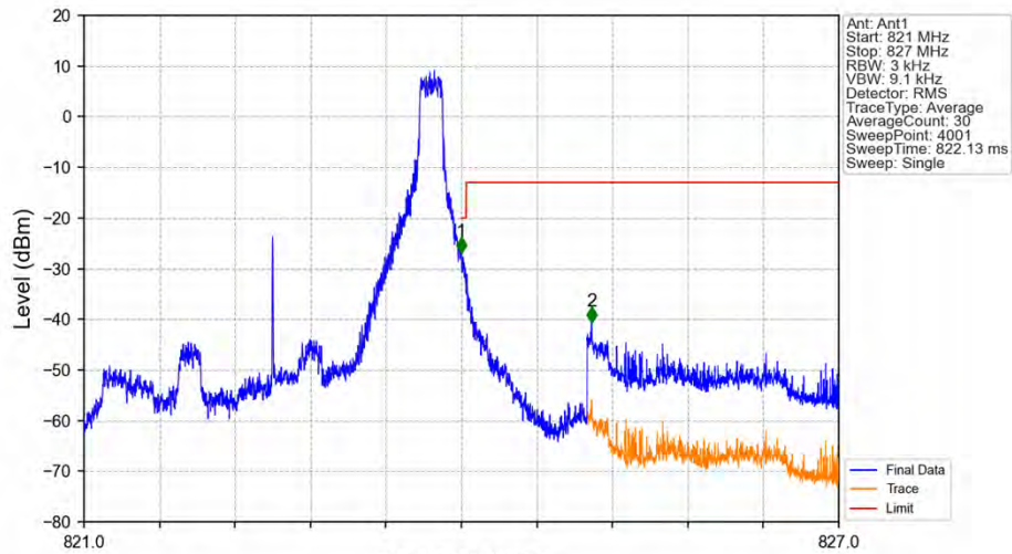
Band26a_3MHz_QPSK_HCH_822.5MHz_RB_1_14_NTNV
