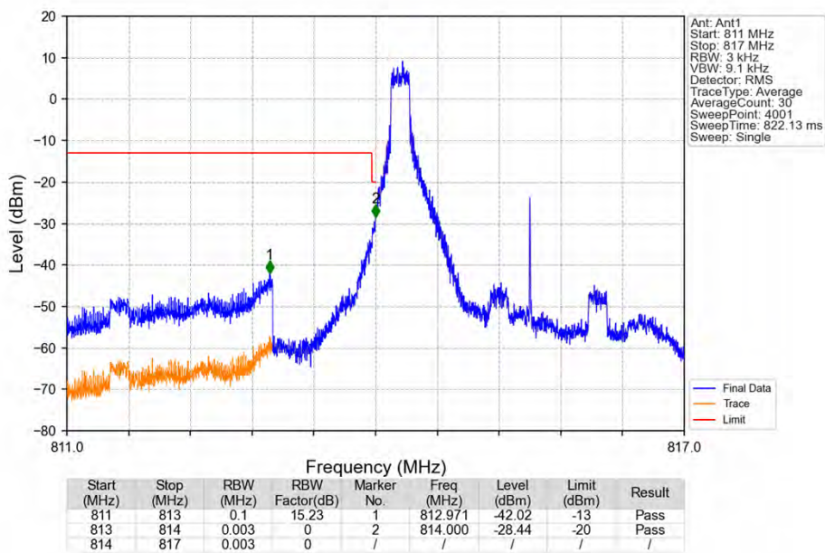
Band26a_3MHz_16QAM_LCH_815.5MHz_RB_1_0_NTNV
