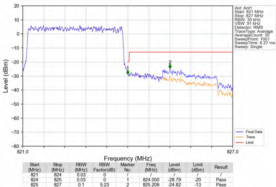
Band26a_3MHz_QPSK_HCH_822.5MHz_RB_15_0_NTNV
