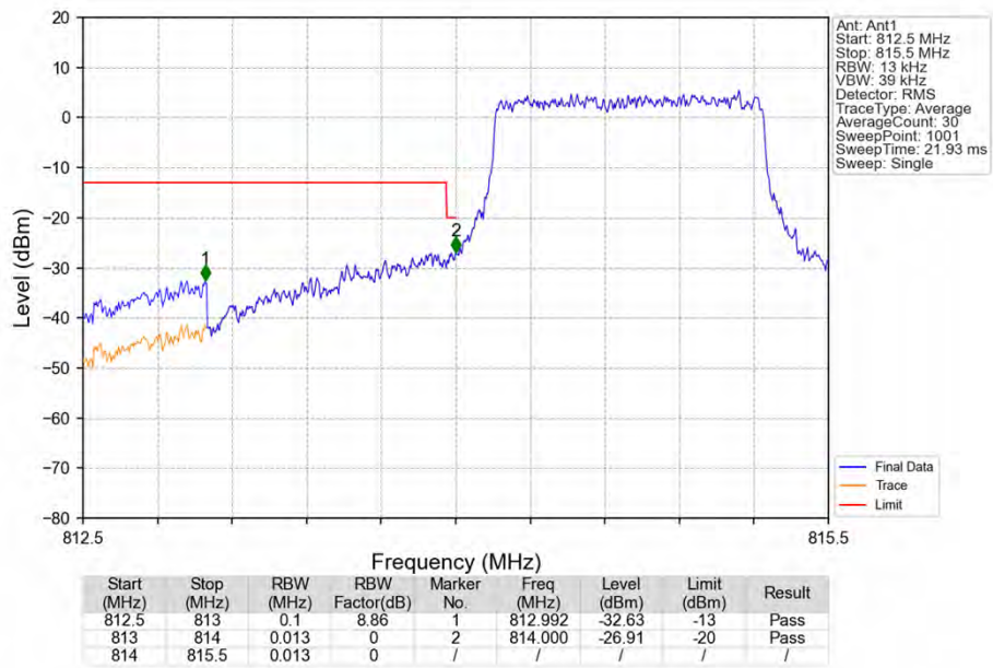
Band26a_1.4MHz_16QAM_LCH_814.7MHz_RB_6_0_NTNV
