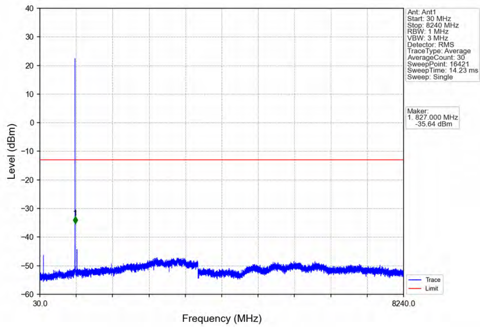
Band26a_1.4MHz_QPSK_HCH_823.3MHz_RB_1_5_NTNV
