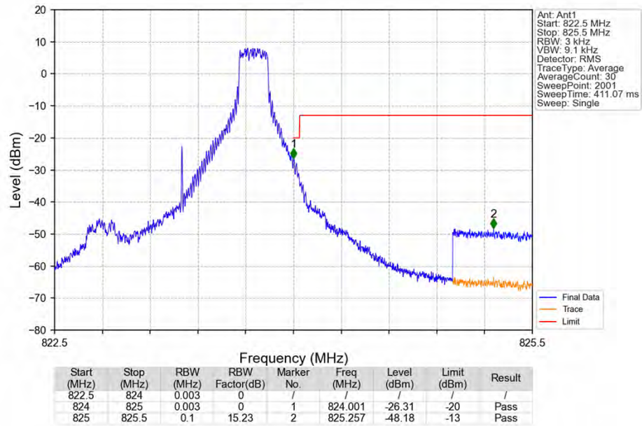
Band26a_1.4MHz_QPSK_HCH_823.3MHz_RB_1_5_NTNV
