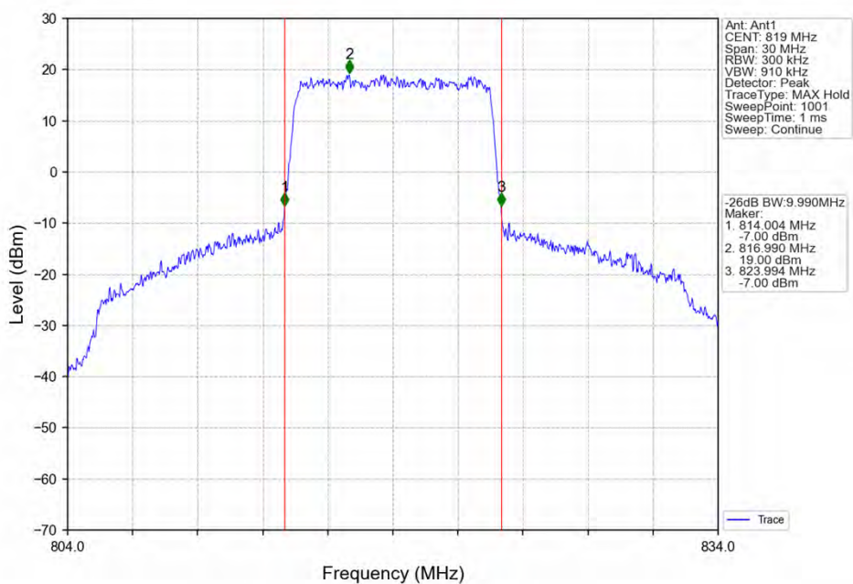
Band26a_10MHz_16QAM_MCH_819MHz_RB_50_0_NTNV
