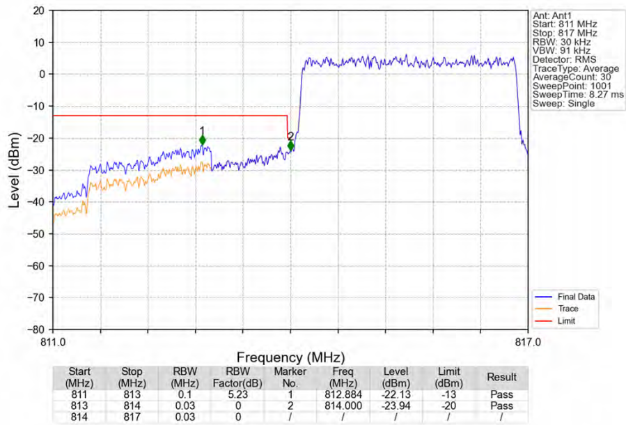
Band26a_3MHz_QPSK_LCH_815.5MHz_RB_15_0_NTNV
