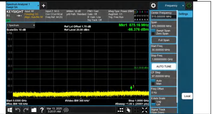
Band38-5MHz-QPSK-38000-1RB#24-30~1000-PASS
