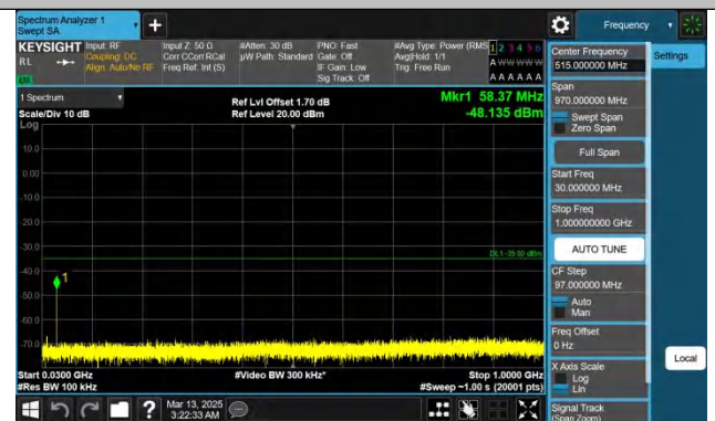
Band38-5MHz-QPSK-38225-1RB#24-30~1000-PASS
