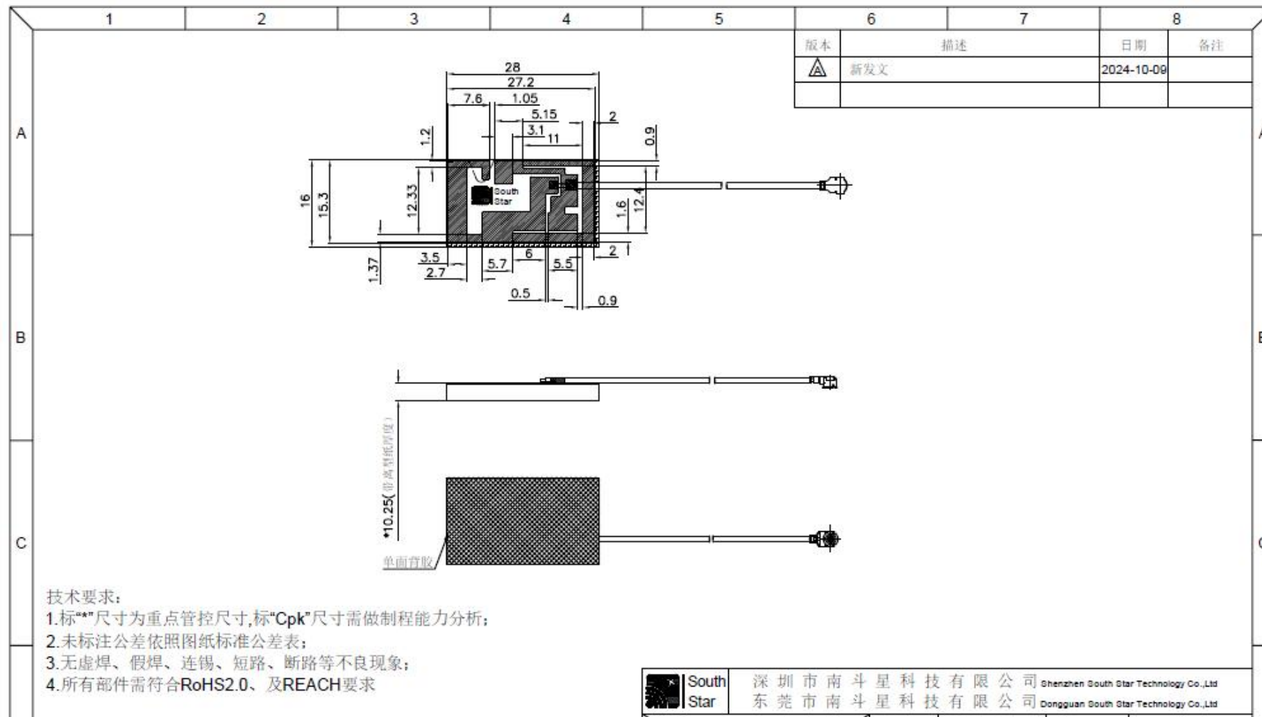
Antenna Drawing
