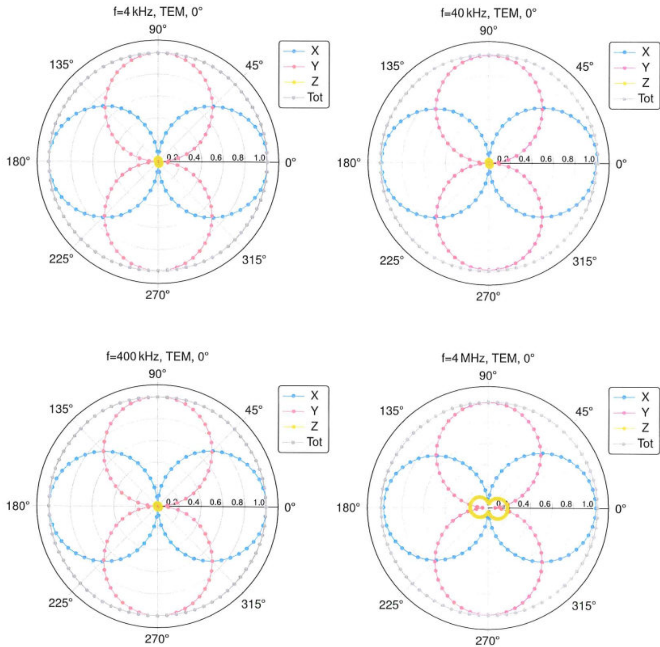
H-Field Receiving Pattern ( \phi ), \vartheta = 0^\circ
