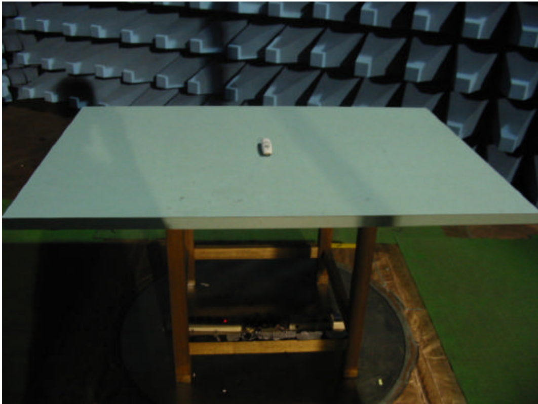
The Test configuration of Front view of y-axis
