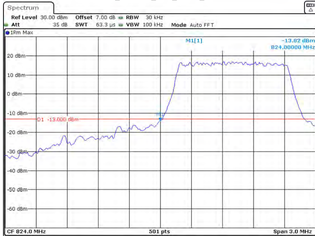
Band 5_1.4 MHz_Low_QPSK_RB6#0
