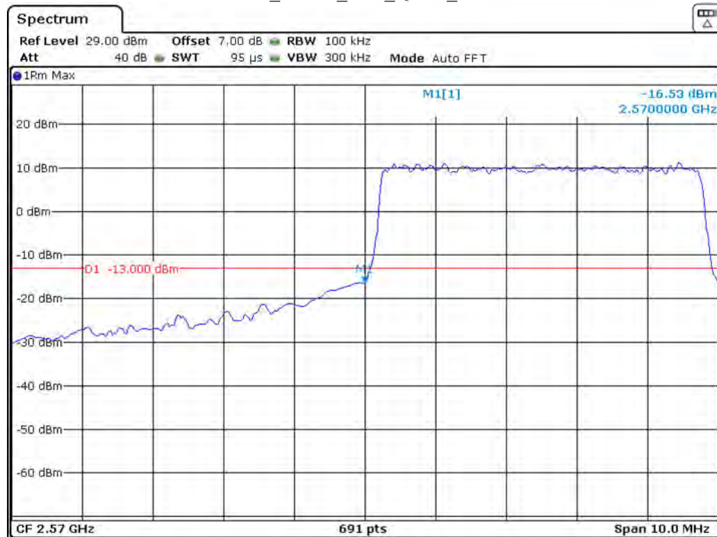
Band 38_5 MHz_Low_QPSK_RB25#0
