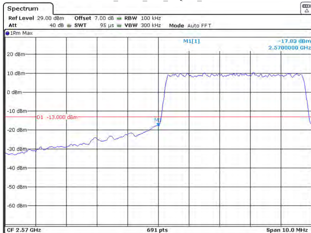
Band 38_5 MHz_Low_16QAM_RB25#0
