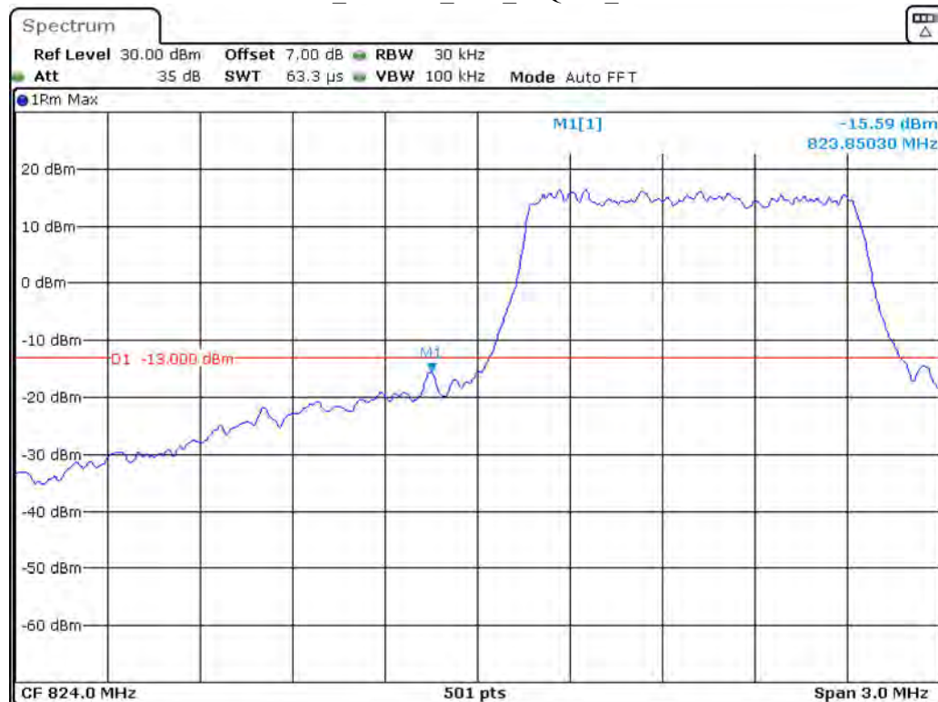
Band 5_1.4 MHz_Low_16QAM_RB6#0
