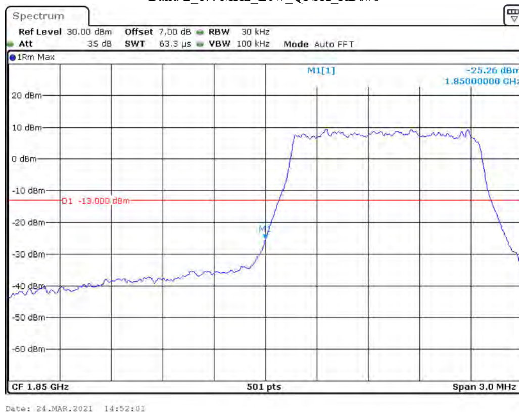
Band 2_1.4 MHz_Low_QPSK_RB6#0
