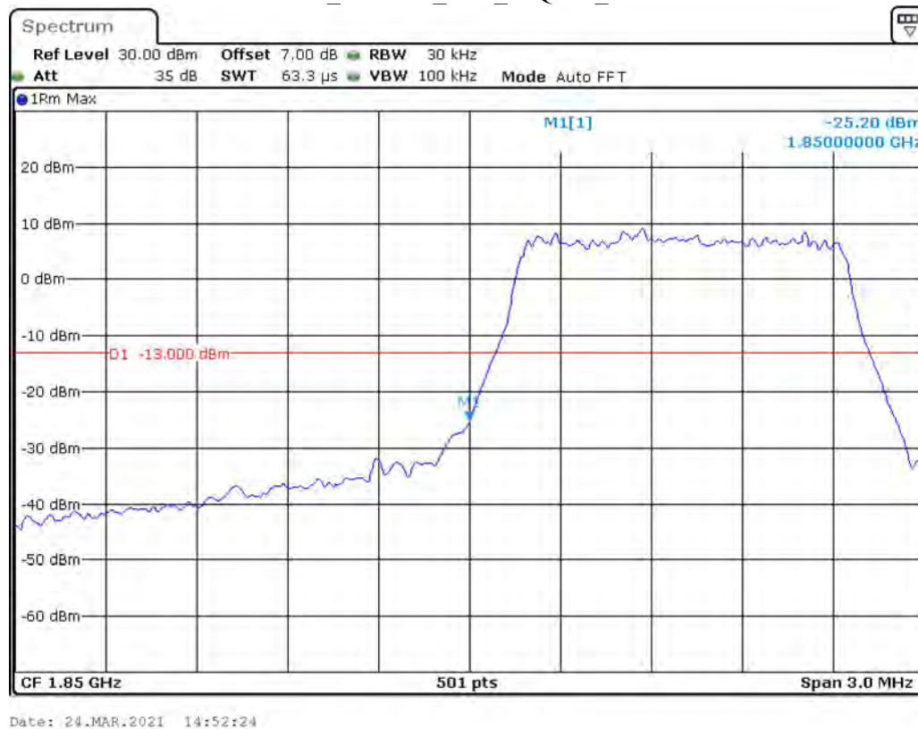
Band 2_1.4 MHz_Low_16QAM_RB6#0
