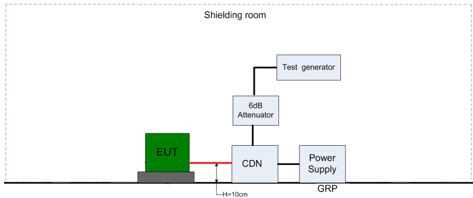
Figure 4. Test set-up of immunity to continuous conducted interference
