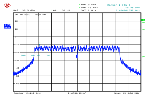
g_2412MHz_Chain 0 -10.48dBm/3kHz
