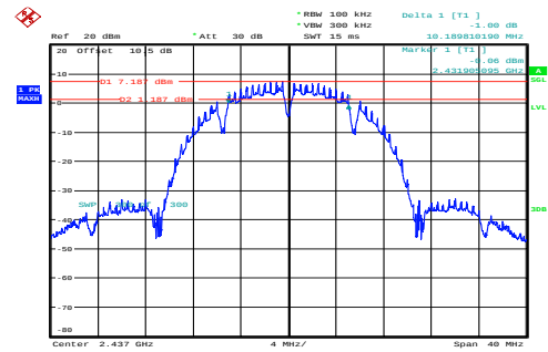
b_2437MHz_Chain 0 10.190MHz
