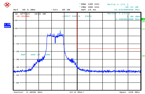
g_2462MHz_Chain 0 40.21dB
