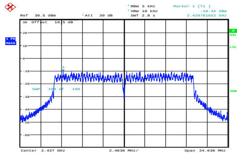
g_2437MHz_Chain 0 -10.42dBm/3kHz
