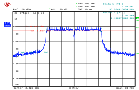
n40_2422MHz_Chain 0 35.884MHz
