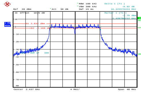
n20_2437MHz_Chain 0 16.424MHz
