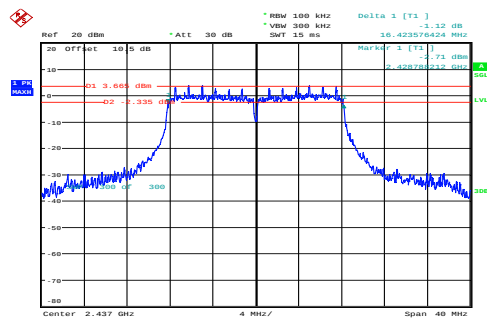
g_2437MHz_Chain 0 16.424MHz
