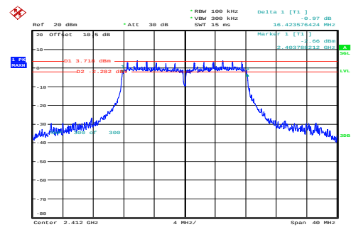
g_2412MHz_Chain 0 16.424MHz
