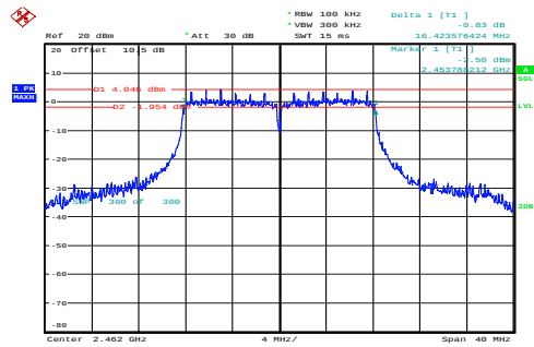
n20_2462MHz_Chain 0 16.424MHz
