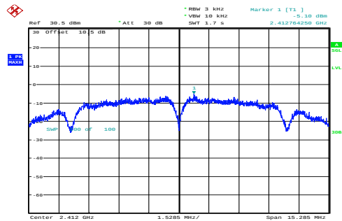
b_2412MHz_Chain 0 -5.10dBm/3kHz
