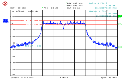
n20_2412MHz_Chain 0 16.424MHz
