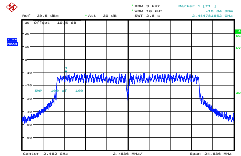
g_2462MHz_Chain 0 -10.04dBm/3kHz
