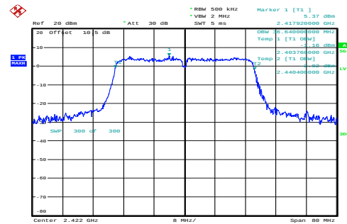
n40_2422MHz_Chain 0 36.640MHz
