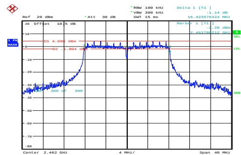
g_2462MHz_Chain 0 16.424MHz
