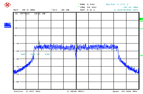
n20_2437MHz_Chain 0 -10.41dBm/3kHz
