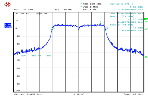
n20_2437MHz_Chain 0 16.640MHz
