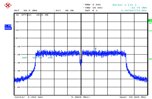
n40_2452MHz_Chain 0 -13.73dBm/3kHz
