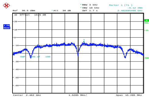
b_2462MHz_Chain 0 -6.12dBm/3kHz
