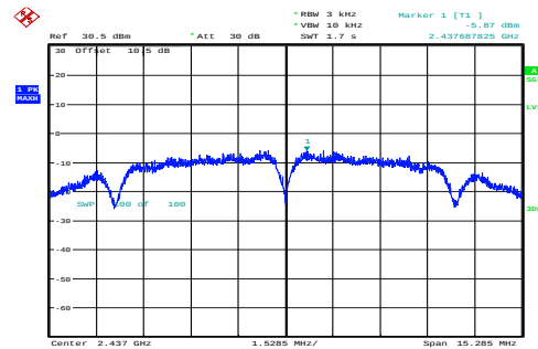
b_2437MHz_Chain 0 -5.87dBm/3kHz
