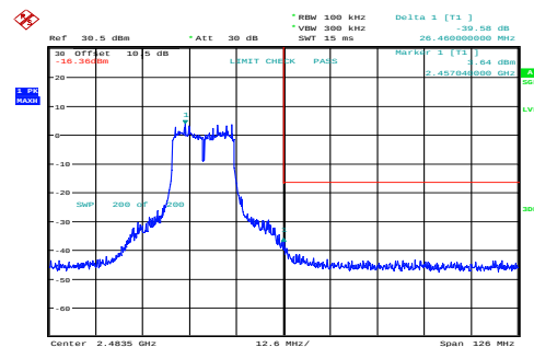
n20_2462MHz_Chain 0 39.58dB
