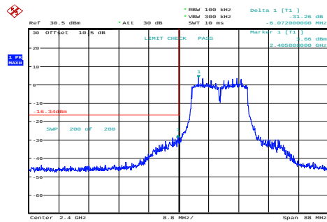
g_2412MHz_Chain 0 31.26dB
