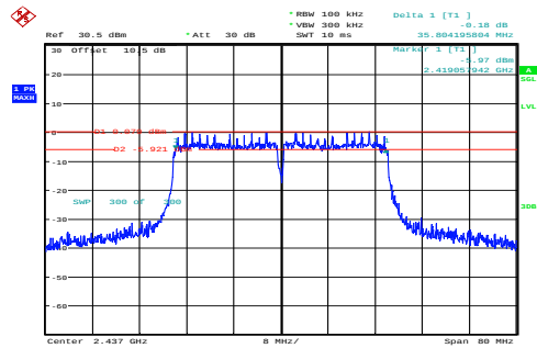
n40_2437MHz_Chain 0 35.804MHz
