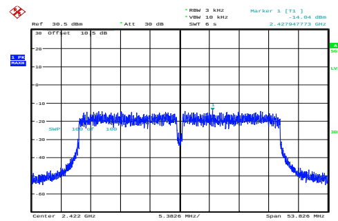
n40_2422MHz_Chain 0 -14.04dBm/3kHz
