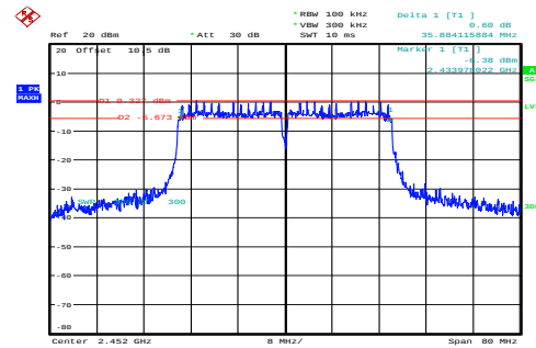
n40_2452MHz_Chain 0 35.884MHz
