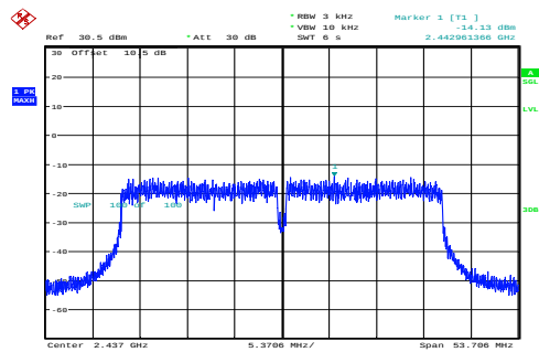
n40_2437MHz_Chain 0 -14.13dBm/3kHz
