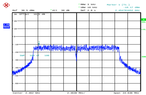
n20_2462MHz_Chain 0 -10.17dBm/3kHz
