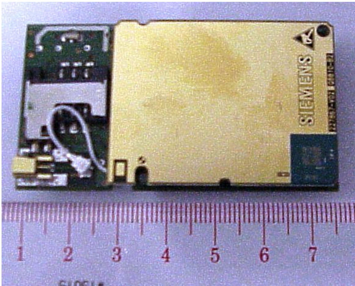
MTSMC-G with TC63 component side
