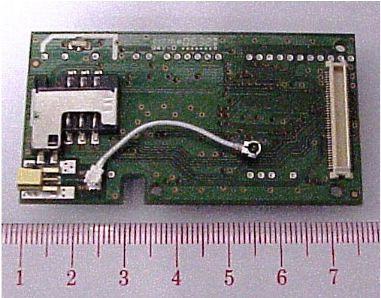
MTSMC-G component side
