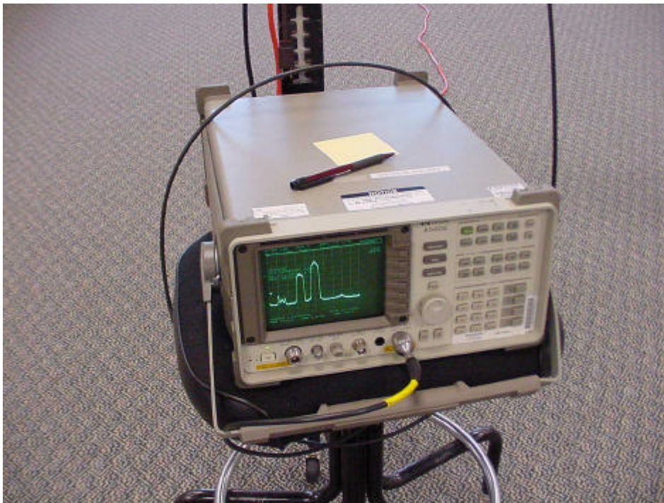
Figure 5. Example of Spectrum Analyzer Display of Base Station Signals for Stable Operation of the SSR
